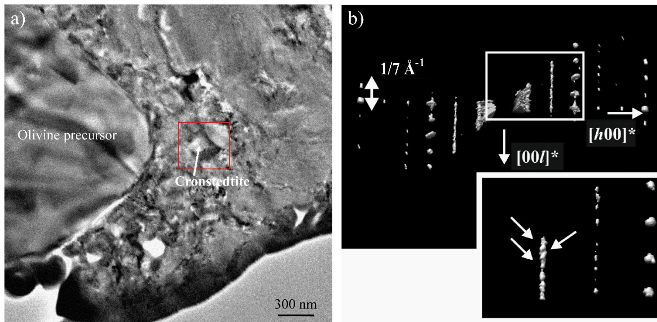
Figure 4. (a) TEM image of a cronstedtite crystal formed close to the remnant of a pseudomorphised olivine. (b) Section of the 3D reconstructed diffraction volume of a sub-micrometric crystal of partially disordered 3T cronstedtite. This section corresponding to (h0l_{\text{hex}})^* plane and is obtained using UCSF Chimera software. In the down-right part of the panel is shown a higher-threshold zoom of the area marked by the white square. Reflections and intensity maxima corresponding to a periodicity of about 21 \text{ \AA} are indicated along the [10l]^* row.
