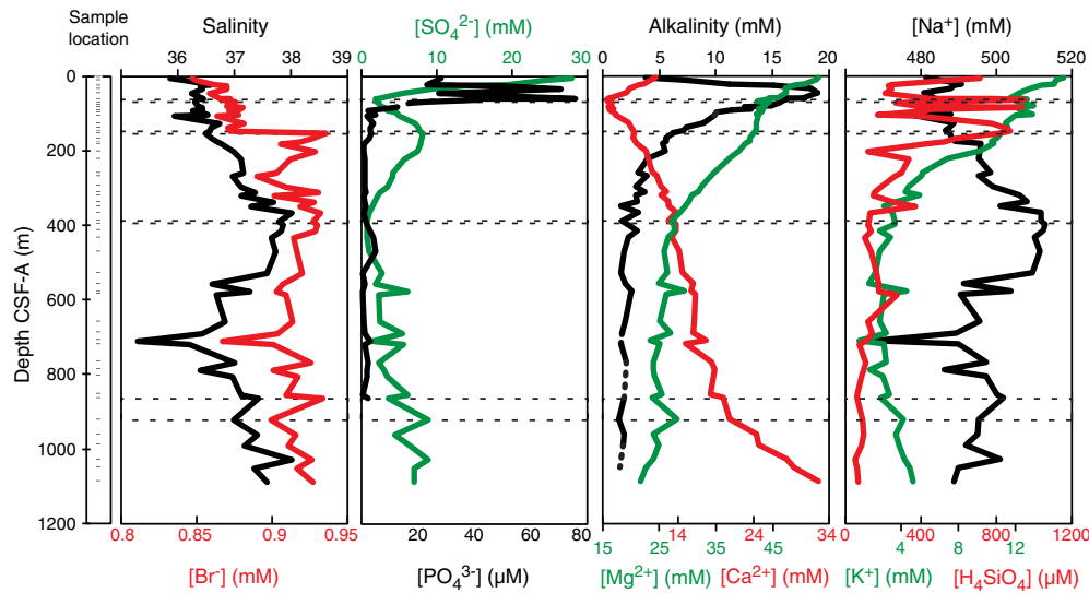
Figure F22. Variations of salinity, bromide, sulfate, phosphate, alkalinity, magnesium, calcium, sodium, potassium, and silicon concentrations in interstitial waters, Site U1451.
