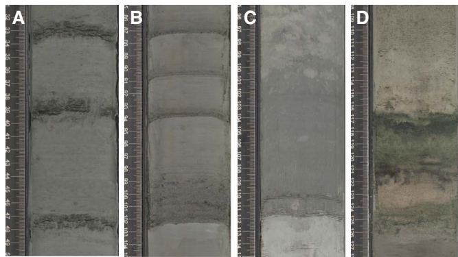
Figure F8. Hole U1451A features. A. Bioturbated clay with bioturbated very thin silt layers (2H-1, 30–50 cm). B. Mud turbidite sequences consisting of repeated lower silt to upper clay units (10H-1, 85–105 cm). C. Structureless to bioturbated clay (100–112 cm) intercalated with calcareous clay (28H-1 95–115 cm). D. Volcanic ash layer (13F-2, 116–126 cm) overlain by calcareous clay (108–128 cm); dark green color indicates diagenetic alteration of volcanic glass.
