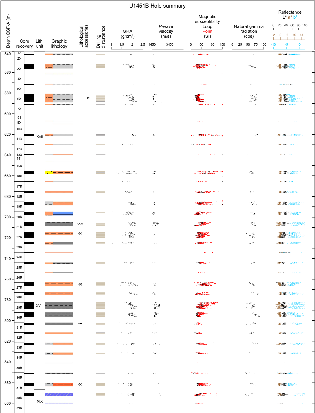
Figure F5. Lithostratigraphic summary, Hole U1451B. For legend, see Figure F5 in the Expedition 354 methods chapter (France-Lanord et al., 2016a). For a larger version of this figure, see LITHOSTRAT in Supplementary material . (Continued on next page.)
