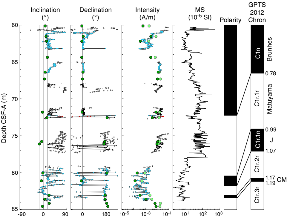
Figure F20. NRM of archive section halves and discrete samples after 20 mT AF demagnetization, Cores 354-U1451A-11F through 15F. These cores were deposited during the early Brunhes and late Matuyama, with the short normal intervals representing the Jaramillo (J) and Cobb Mountain (CM) Subchrons. Circles = measurements do not meet quality criteria. Blue dots = calcareous clay, black dots = other lithology, green dots = discrete samples. Declination is rotated and illustrates magnetostratigraphic interpretation. A single vertical axis rotation was applied to the entire core so that points interpreted as normal polarity plot near the 0° line. Intensity = intensity of magnetization after 20 mT AF demagnetization. Magnetic susceptibility (MS) = point measurements on archive section halves. Polarity: black = normal, white = reversed, gray = uncertain. Geomagnetic polarity timescale (GPTS) of Gradstein et al. (2012).
