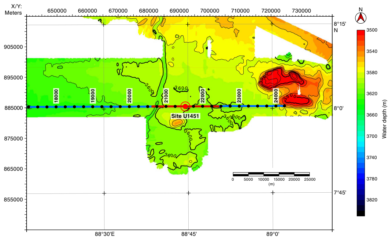
Figure F1. Bathymetric and track chart, Site U1451. Two knolls rise ~50 and ~200 m above the fan surface. A minor straight channel passes ~10 km west. Projection is UTM Zone 45N. Multibeam bathymetry was acquired during R/V Sonne Cruises SO125 and SO188. Blue line = seismic Line SO125-GeoB97-027 with common depth point annotation. Contour interval is 20 m. Portions of seismic data are shown in Figures F2 (red line, 22 km) and F3 (14 km).
