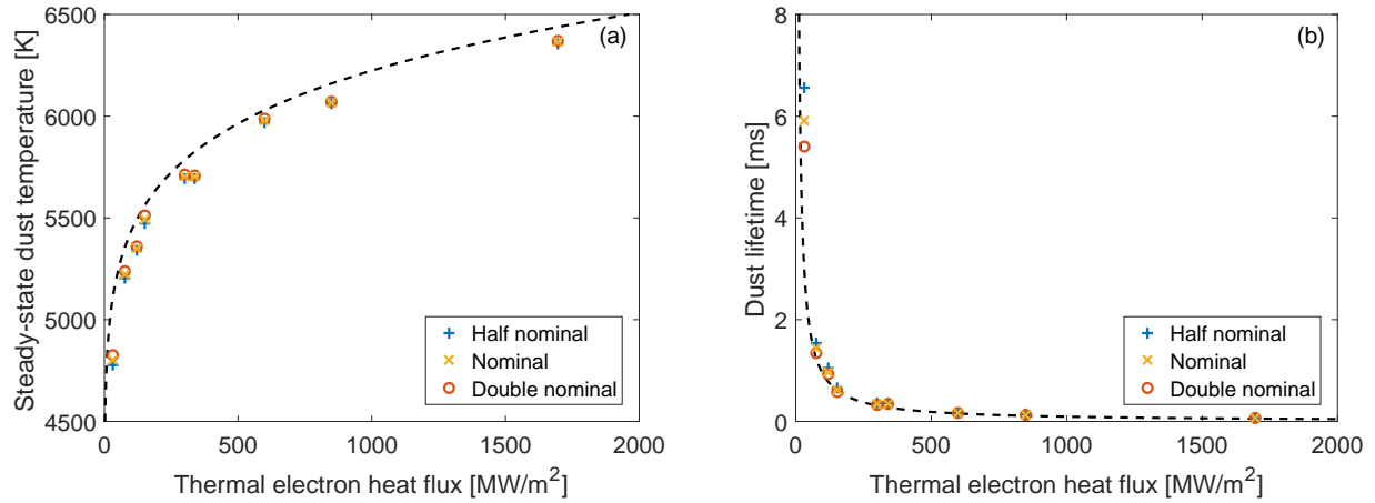
Figure 11. MIGRAINE simulations of a W grain with initial radius 1 \mu\text{m} and temperature 300 K in a uniform plasma whose electron density n_e = 2\text{--}10 \times 10^{20} \text{ m}^{-3} and temperature T_e = 2\text{--}10 \text{ eV} were scanned independently. The intensity of thermionic emission was varied between half and twice its nominal value (5). The steady-state dust temperature (a) and dust lifetime (b) are plotted as a function of the thermal electron heat flux as defined by (3). Approximated OML scalings (2) and (4) are plotted as black dashed curves.
