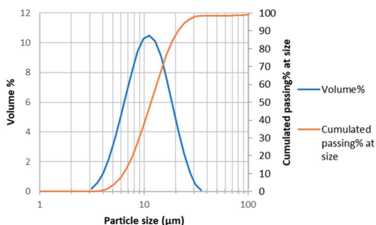
Fig. 1 Particle size distribution of NMC 811.
