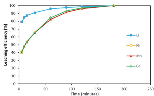
Fig. 3 Leaching kinetics of NMC 811 in 4 \text{ mol } L^{-1} HCl at S/L = 20 \text{ g } L^{-1} and 25 \text{ }^{\circ}\text{C} .
