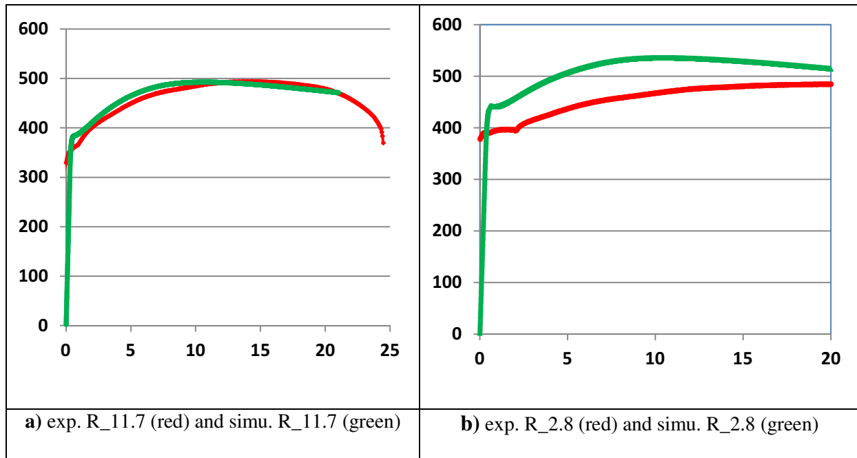
Figure 4: Experimental and simulated tensile curves ( \sigma_{eng} (MPa) versus \epsilon_{eng} (%))
