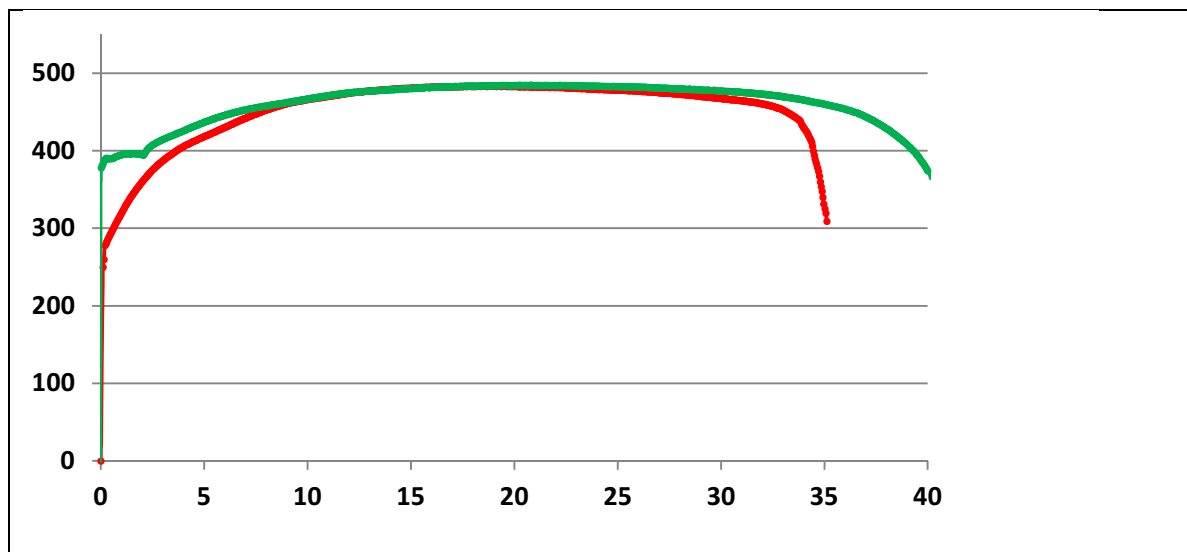
Figure 3: Engineering stress (MPa), \sigma_{eng} , versus engineering strain in %, \varepsilon_{eng} , for the two specimens R_21.3 (red curve) and R_2.8 (green curve).
