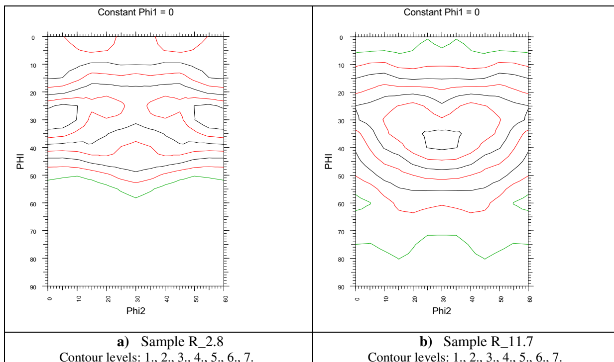
Figure 2: Section \text{Phi}1=0^\circ of the ODF for two specimens a) sample R_2.8 b) sample R_11.7
