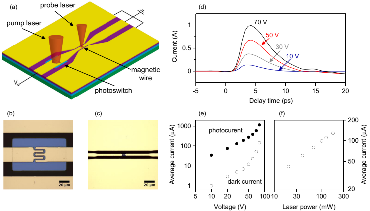
FIG. 1. Device for electrically induced ultrafast demagnetization experiments. (a) Schematic of the electrical demagnetization experiments. The Auston switch is illuminated with a 1.5 nJ laser pulse while biased between 10 and 80 V. The magnetization of the magnetic wire is monitored via TR-MOKE. (b) Optical image of the Auston switch. During illumination, photoexcited carriers in the low-temperature GaAs substrate conduct current across the gap, generating a transient electrical pulse that propagates along the waveguide towards a ferromagnetic section of the centerline. (c) Optical image of the CoPt section of the waveguide. (d) Temporal profile of the current pulse generated by the photoswitch, as measured with a Proteomics probe positioned between the photoswitch and the CoPt wire. (e) Average current across the device with 160 mW of laser power irradiating the photoswitch. The filled circles correspond to measurements while the photoswitch was irradiated with 1.5 nJ laser pulses at a rate of 80 MHz (photocurrent). Open circles are current measurements on the device without laser irradiation (dark current). A rapid increase in dark current occurs as the bias voltage across the photoswitch approaches the breakdown voltage of the device, \sim 90 V. (f) Dependence of the average current on average laser power with a bias voltage of 30 V.
