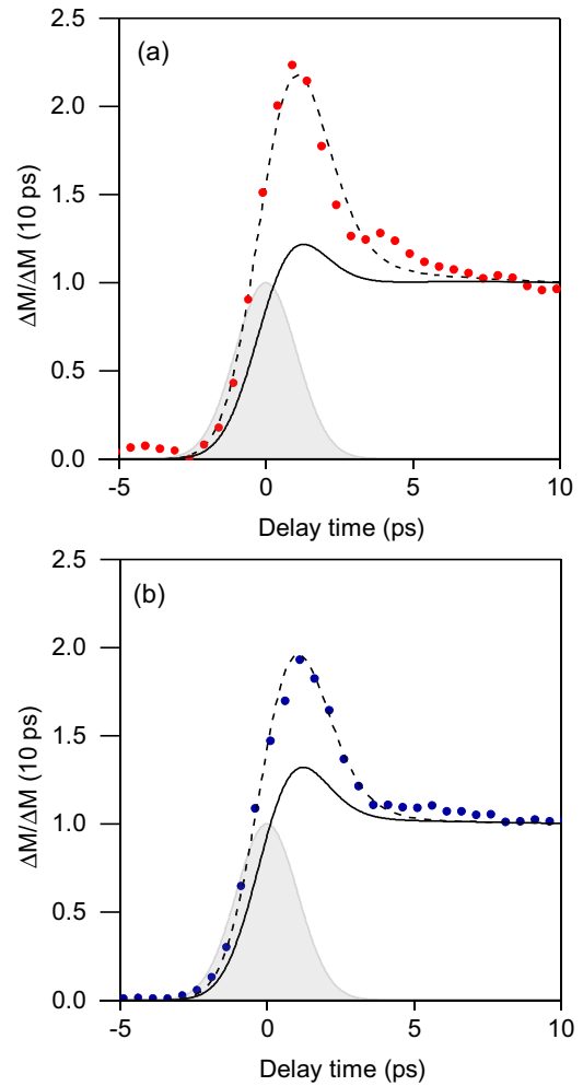
FIG. 2. Optically induced demagnetization of (a) Pt/CoPt and (b) CoPt samples. The markers are normalized TR-MOKE measurements of the demagnetization of the Pt/CoPt and CoPt samples following optical absorption of \sim 0.2 and 0.7\ \text{J m}^{-2} . The shaded region represents the power vs time of the irradiating laser. The solid lines are a three-temperature model prediction for the magnetization dynamics with an electron phonon energy transfer coefficient predicted by scattering theory, g_{ep} = 15 \times 10^{17}\ \text{W m}^{-3}\ \text{K}^1 . To explain the demagnetization data on picosecond scales with a thermal model, the net energy-transfer coefficient must be reduced from the theoretical value to g_{ep} = 7 \times 10^{17}\ \text{W m}^{-3}\ \text{K}^1 , see dashed lines.
