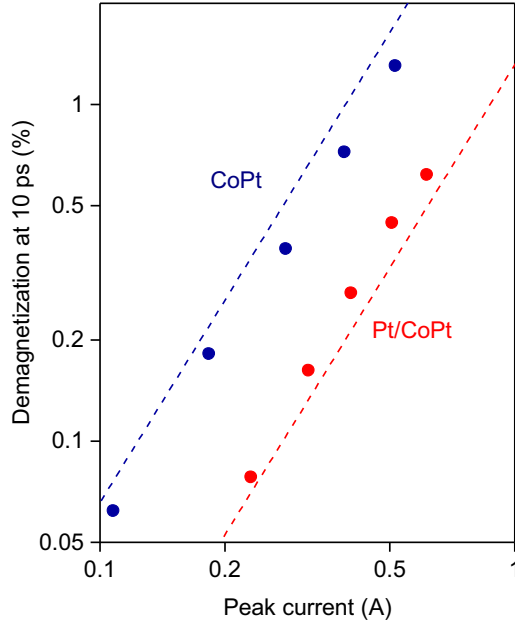
FIG. 4. Demagnetization vs amplitude of the current pulse. Markers are TR-MOKE measurements of the demagnetization 10 ps after the electrical pulse heats the Pt/CoPt (red) and CoPt (blue). The dashed line are the predictions of our thermal model, using the value of (1/M)dM/dT derived from optical demagnetization experiments and our calculation of the energy absorbed by the electrons via joule heating.
