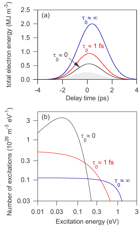
FIG. 6. Nonthermal model predictions for the evolution of the electron energy in response to a 2.6 \text{ ps} optical heat pulse. (a) Total energy stored by electronic excitations vs time for no electron-electron scattering ( \tau_0 = \infty ), strong electron-electron scattering ( \tau_0 = 0 ), and realistic electron-electron scattering rates for Pt ( \tau_0 = 1 \text{ fs} ). The gray region represents the temporal profile of the optical heating term, A(t) , with arbitrary units. (b) Predictions for the number of excitations across various excitation energies at zero time delay. Despite the picosecond time scale of the heating, the distribution of energy predicted by Eq. (3) is nonthermal for finite or zero electron-electron scattering.
