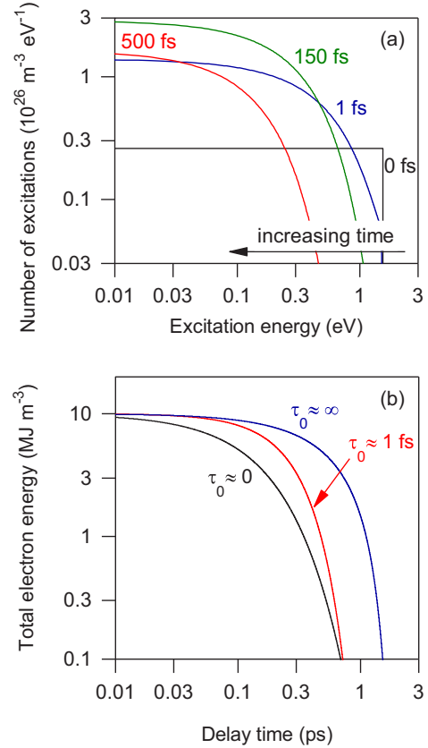
FIG. 5. Nonthermal model predictions for the evolution of the electron energy in time. (a) Relaxation of the excited distributions due to electron-phonon and electron-electron scattering with \tau_{ep} = 20 fs and \tau_0 = 1 fs. (b) Total energy stored by electronic excitations vs time following impulsive heating for no electron-electron scattering ( \tau_0 = \infty ), strong electron-electron scattering ( \tau_0 = 0 ), and realistic electron-electron scattering rates for Pt ( \tau_0 = 1 fs).
