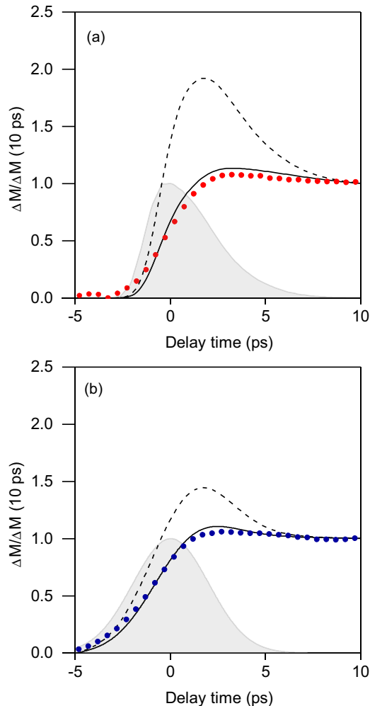
FIG. 3. Electrically induced demagnetization in (a) Pt/CoPt and (b) CoPt samples. Markers are normalized TR-MOKE measurements of the magnetization of the samples after heating by an electrical pulse with \sim 0.5 A peak amplitude. The shaded region represents the power profile of the electrical pulse, as deduced from Proteomics probe measurements. The heating time scales are slightly different for the two samples due to differences in the Auston switch devices. The solid lines are three-temperature model predictions for the demagnetization with the theoretically calculated value of g_{ep} = 15 \times 10^{17} \text{ Wm}^{-3} \text{ K}^1 . For comparison with the optical experiments, the dashed lines show predictions with a reduced electron-phonon energy transfer coefficient of g_{ep} = 7 \times 10^{17} \text{ Wm}^{-3} \text{ K}^1 . A higher rate of energy transfer between electrons and phonons in the electrical heating experiments explains why there is no recovery of the magnetization in the picoseconds following electrical heating.
