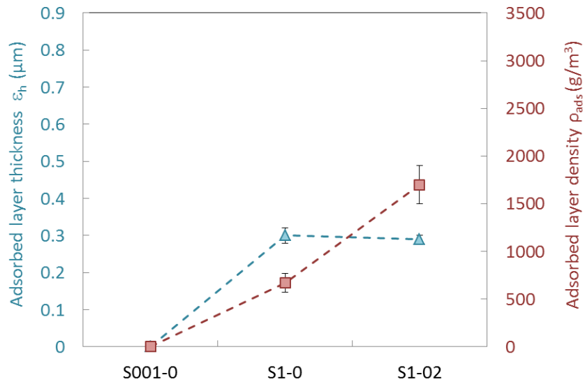
Figure 17: Estimations of the polymer adsorbed layer thicknesses and densities for the tests performed in the quartz porous media for the various salinities investigated.
