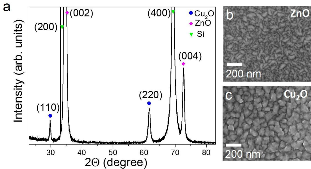
Figure 2. (a) X-ray diffractogram of the \text{Cu}_2\text{O}/\text{ZnO} heterojunction on a Si substrate. (b) Top-view SEM micrograph of the ZnO (b) and \text{Cu}_2\text{O} (c) films.
