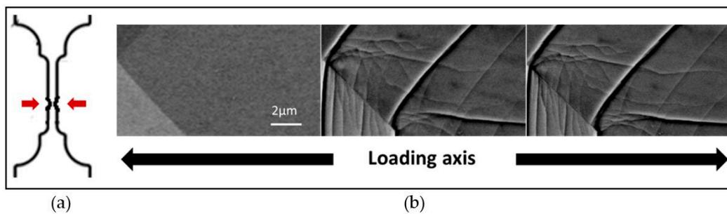
Figure 6. (a) Local section reduction to create high-strained zones (b) BSE micrographs in channeling condition post mortem test showing dislocation networks and slip lines forming and evolving during plastic deformation.
