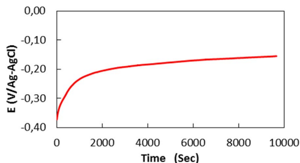
Fig. 4. Evolution of open circuit potential of nano-peened AISI 304L immersed in filtrate at 25 \text{ }^\circ\text{C} , without mechanical loading.
