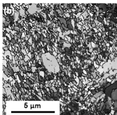
Fig. 3. Nanosized ferrite grains at the top layer of the nano-peened 304L sample (a) BSE micrograph close to the top surface, (b) Inverse Pole Figure (IPF) EBSD map of the ferrite phase - the map was acquired in the middle of the 60\ \mu\text{m} thick top layer.
