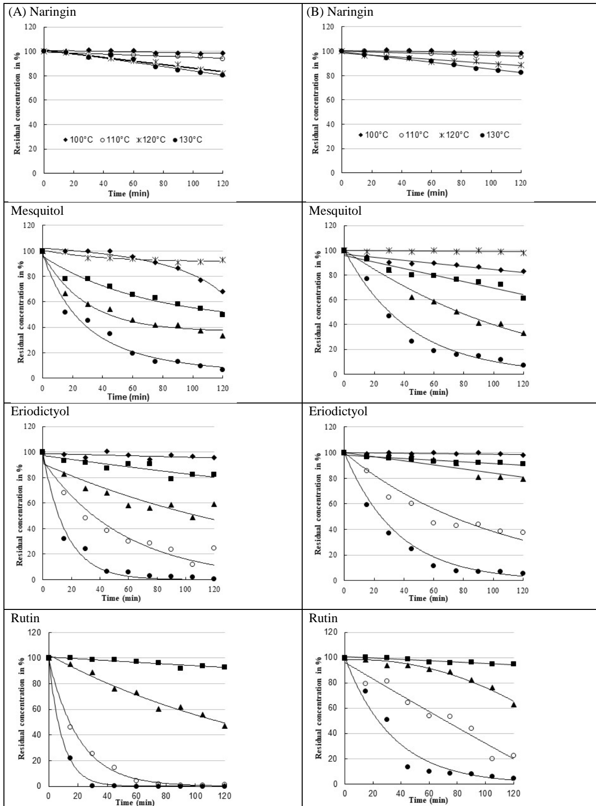
Figure 3. Degradation kinetics of flavonoids at different temperatures over 2 h (×30°C ◆50°C ■70°C ▲90°C ○110°C ●130°C)
