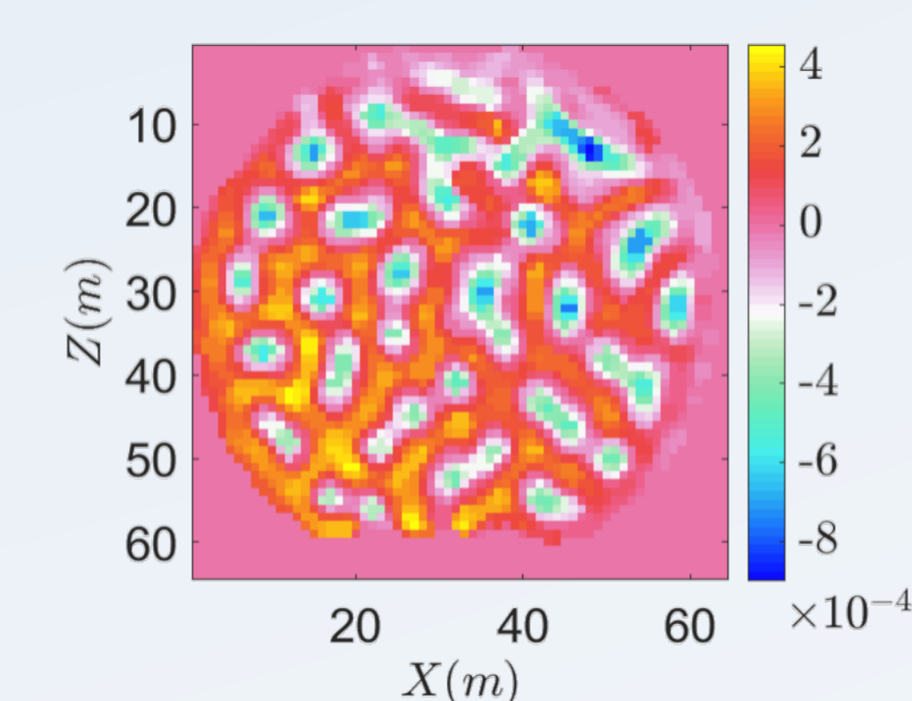
Vertical velocities in butyl stearate (horizontal slice)
