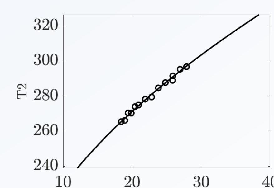
Calibration curve of T2 as a function of temperature.
