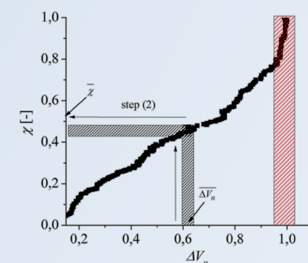
Evolution of the ice fraction \chi with the normalized ice volume
