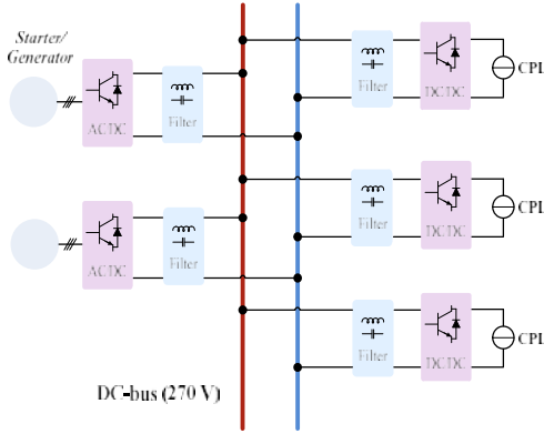
Fig. 1. Typical DC microgrid of more electric aircraft.
