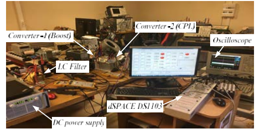
Fig. 4. Experimental bench.
