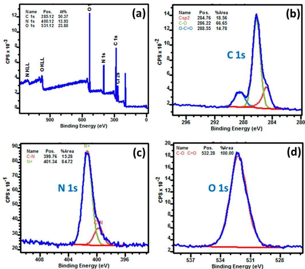
Figure 3. XPS data of GQDs (a) full-scan XPS spectrum, (b) C 1s spectrum, (c) N 1s spectrum, and (d) O 1s spectrum.
