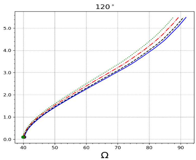
Figure 6. The amplitude-frequency relation with different levels porosity ( e_p ) for hinged-hinged curved beams with L/r_g = 100 : a) w_{gpl} = 0.0\% , b) w_{gpl} = 0.25\% c) w_{gpl} = 0.75\% .
