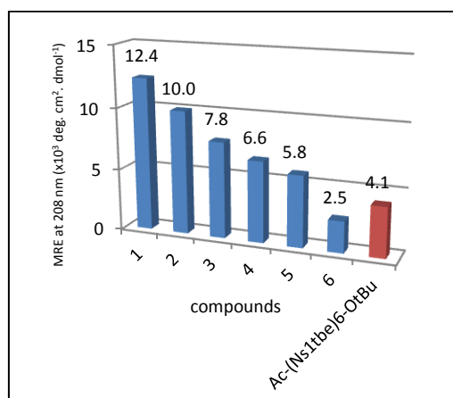
Figure 4. MRE values of hexamers 1-6 and reference compound Ac-(Ns1tbe) 6 at 208 nm in MeOH
