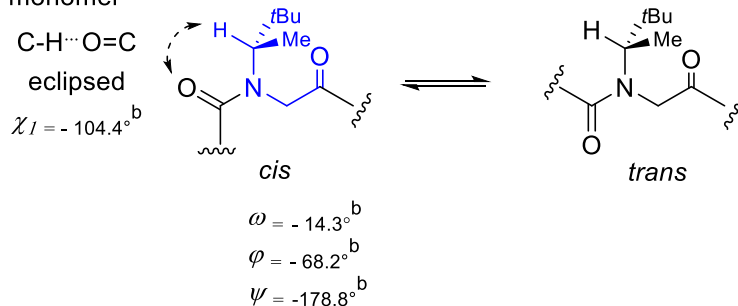
Figure 1. Structure and conformational characteristics of the NtBu and Ns1tbe peptoid residues used in this study (drawn in blue), see table 2 for the dihedral angles definition. a Measured for the central residue of the crystal structure of H-( NtBu ) 5 -OBn. 30 b Measured for the central residue of the crystal structure of Ac-( Ns1tbe ) 5 -OtBu 16 . The \chi_1 angles have been measured for each tBu NC \beta methyl carbon in case of the representative NtBu monomer; the tBu NC \beta has been used for measuring the \chi_1 angle (-104.4) in case of the representative Ns1tbe monomer.
