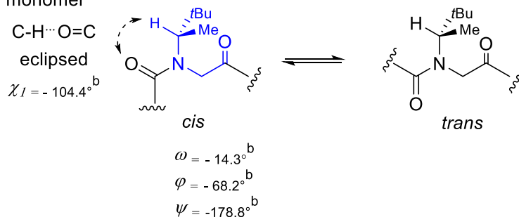
Figure 1. Structure and conformational characteristics of the NtBu and Ns1tbe peptoid residues used in this study (drawn in blue), see table 2 for the dihedral angles definition. a Measured for the central residue of the crystal structure of H-( NtBu ) 5 -OBn. 30 b Measured for the central residue of the crystal structure of Ac-( Ns1tbe ) 5 -OtBu 16 . The \chi_1 angles have been measured for each tBu NC \beta methyl carbon in case of the representative NtBu monomer; the tBu NC \beta has been used for measuring the \chi_1 angle (-104.4) in case of the representative Ns1tbe monomer.
