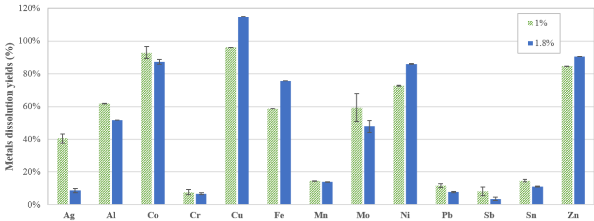
Figure 14: Bioreaching yields (in %) according to the concentration of solids in the double-stage bioreactor run in continuous mode. Error bars depict uncertainties in the leachate analysis.
