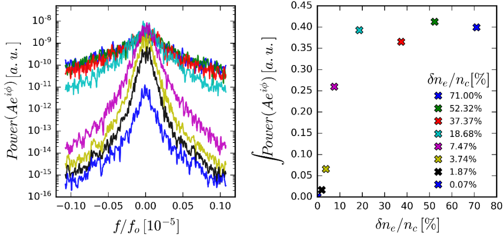
Figure 3. Left: power spectra of the reflectometry complex amplitude signals Ae^{i\phi} obtained from simulations with fixed probing frequency f_0 = 30 GHz over a turbulence level scan of GEMR data. Right: total integrated power of the corresponding spectra on the left panel, against the turbulence level.
