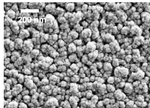
Figure 2 SEM micrograph of NCD film deposited on S1 sample (ZnO/Si).
