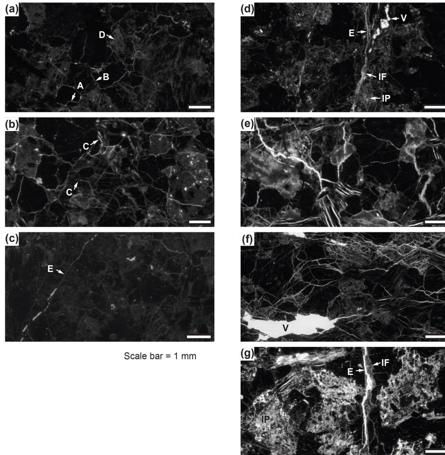
Figure 7. UV-fluorescent light photomicrographs showing microstructural position of connected porosity. Representative situations for fresh granite and pink granite near a single fracture (a), for fractured and weakly altered granite (b), for pink granite in a fracture corridor (c), for green granite (d), for brown granite near a single fracture (e), for brown granite in a fracture corridor (f) and for yellow granite in a fracture corridor (g). D: distributed porosity in plagioclase, B: grain boundary crack, A: intragranular crack, C: cleavage crack, E: intergranular crack, V: cavity, IF: illite infills in fracture and IP: illite aggregate in plagioclase.
