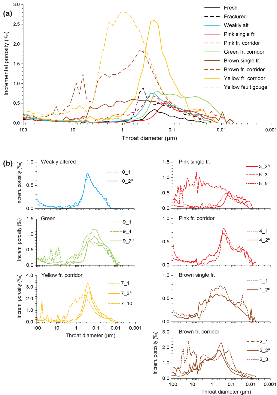
Figure 10. Incremental porosimetric curves showing throat size distributions of the connected porosity of (a) different facies and of (b) specific fracture-related features within the altered facies. From the latter, specimens indexed with “R” were selected as representative of the facies matrix and plotted in (a), compare with Fig. 3. Fr.: fracture, alt.: altered.
