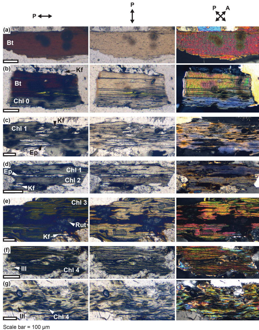
Figure 5. Polarized light photomicrographs showing optical properties of biotite and its alteration products. The double-headed arrows show polarization direction of polarizer (P) and analyzer (A) for each column; (a) biotite and (b) biotite partially replaced by chlorite (Chl 0) in fresh granite; (c) chlorite (Chl 1) in weakly altered granite; (d) chlorite (Chl 1 and Chl 2) in green granite; (e) chlorite (Chl 3) in brown granite; (f, g) chlorite (Chl 4) and illite in yellow granite. Bt: biotite, Kf: K-feldspar, Ep: epidote, Rut: rutile and Ill: illite.
