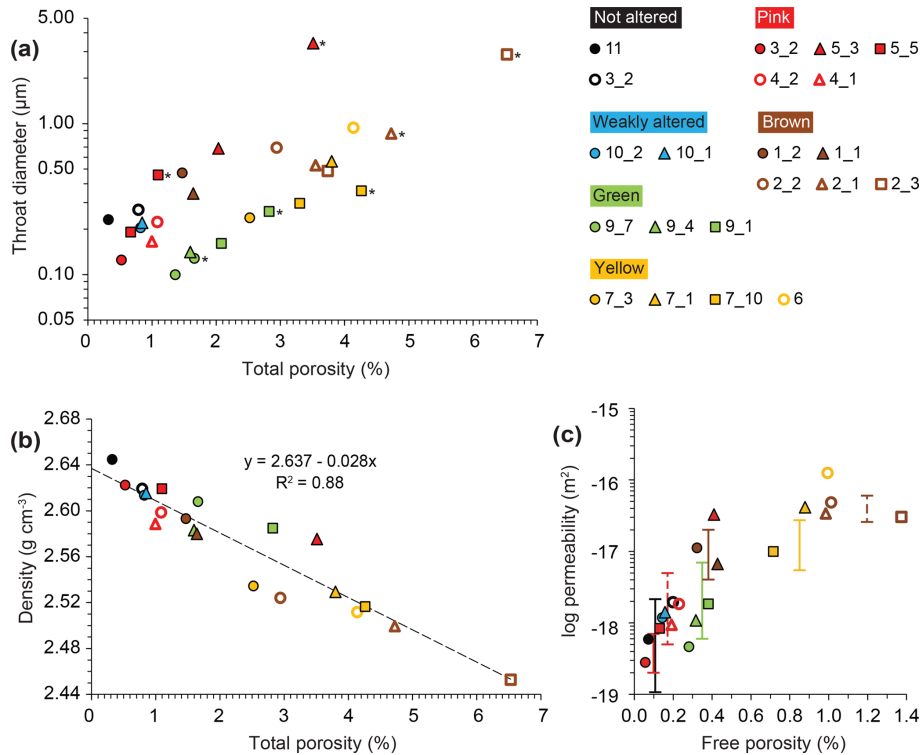
Figure 11. Plots of measured throat diameter, porosity, density and calculated permeability. (a) Volumetric median throat diameter versus total porosity. For all specimens the values were calculated for the throat diameter interval 0.005–5 μm and for specimens with macroscopic voids also for the interval 0.005–300 μm (denoted by an asterisk to the right of the symbols); (b) bulk density versus total porosity. Total porosity calculated for the throat diameter intervals 0.005–5 and 0.005–300 μm for specimens without and with macroscopic voids, respectively; (c) point symbols: permeability calculated after Katz and Thompson (1986, 1987) from the total porosity and median throat diameter (calculated for throat diameter interval 0.005–5 μm) versus free porosity measured by mercury reintrusion (failed for specimen 7_3); bars: intervals of permeability measured by gas permeametry on plugs.
