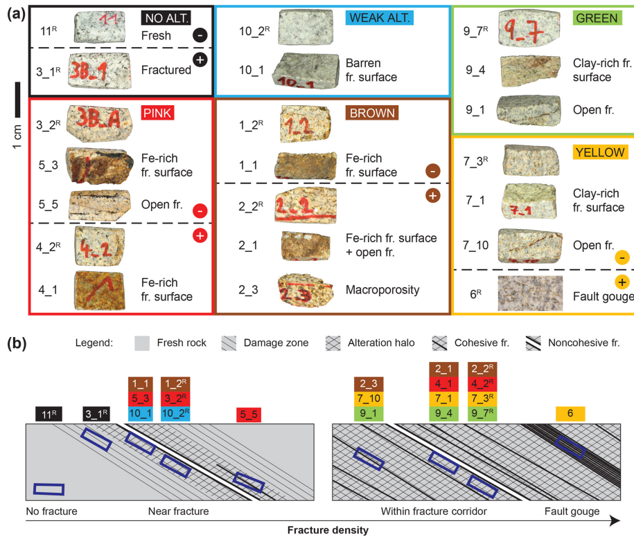
Figure 3. (a) Photographs and parametric description of specimens tested by mercury porosimetry grouped by alteration facies. The dashed lines delimit subgroups of specimens from lower (minus symbol) and higher (plus symbol) fracture density zones; (b) schematic sketch of rock cores and sampled materials showing in a simplified way the position of the specimens within the core samples. Specimens indexed with “R” were selected as representative of the matrix of the facies. Alt.: alteration, fr.: fracture.
