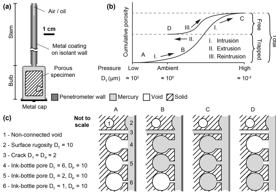
Figure 4. Mercury porosimetry; (a) schematic drawing of a penetrometer (specimen holder); (b) plot of an idealized cumulative porosimetric curve to explain the measurement of connected total, trapped and free porosity by mercury reintrusion, A–D relate to (c); (c) schematic drawings of void spaces in a rock specimen to explain the phenomenon of mercury entrapment with respect to different arrangements of throats in relation to pores. D_T : throat diameter, D_p : pore diameter.
