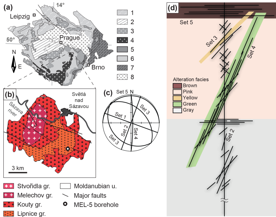
Figure 1. Maps showing the location of the sampled borehole. (a) Simplified geological map of the Bohemian Massif (modified after Franke 2000) 1: Saxothuringian and Lugian, 2: Teplá–Barrandian, 3: Variscan granitoids, 4: Moldanubian batholith, 5: Gföhl assemblage, 6: Drosendorf and Ostrong assemblage, 7: Brunovistulian, and 8: Cretaceous sedimentary cover; (b) geological map of the Melechov pluton (modified after Machek, 2011) with gr. representing granite and u. representing unit; (c) stereoplote (Schmidt projection) of the fracture sets recognized within the Melechov pluton based on Lexa and Schulmann (2006) and Staněk (2013); (d) interpretative schematic sketch of the fracture sets and their structural relationship with respect to the alteration facies distribution within the borehole.
