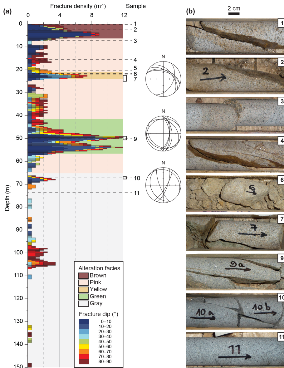
Figure 2. Fracture and alteration setting of samples. (a) Borehole log showing fracture density distribution (modified after Lexa and Schulmann, 2006), macroscopic alteration zones and position of samples. The pole diagrams (Schmidt projection) show orientation of fractures in the vicinity of samples with the depth range defined by the rectangles at the right side of the log (based on the acoustic borehole image, not available for the uppermost 22.5 m); (b) photographs of the samples.
