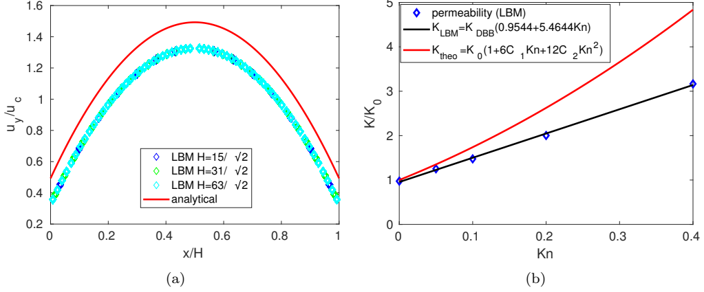
Figure 3: (a) Dimensionless velocity profiles for Poiseuille flow inside the 45^\circ inclined channel with the DBB boundary condition applied at the solid-fluid interface ( \text{Kn} = 0.1 ). (b) Dimensionless permeability of the 45^\circ inclined channel as function of \text{Kn} ( H = \frac{15}{\sqrt{2}} ).
