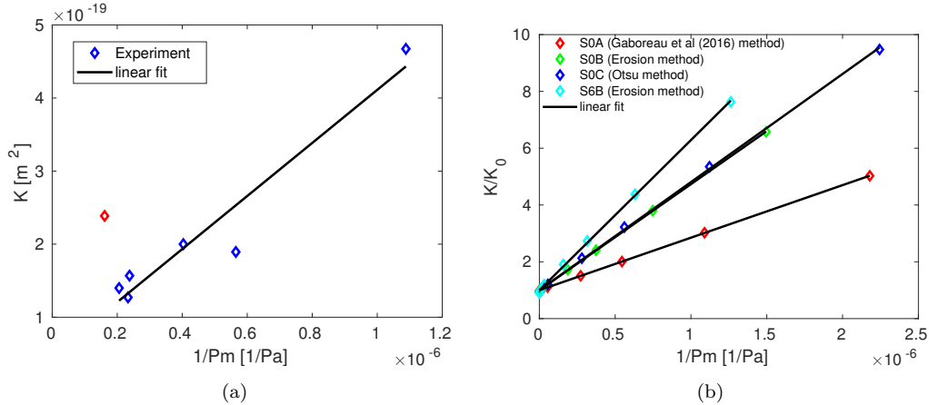
Figure 6: (a) Experimentally measured permeabilities of the compacted illite sample versus the inverse of the mean gas pressure. (b) Dimensionless numerically calculated permeabilities of S0x and S6B sub-samples versus the inverse of the mean gas pressure. Solid lines are linear fits by (2).
