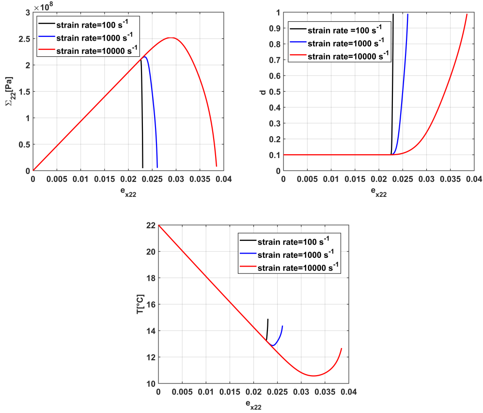
FIGURE 9: Effective stress, damage and temperature for different strain rates : \dot{e}_{x22} = 100 s^{-1} , \dot{e}_{x22} = 1000 s^{-1} and \dot{e}_{x22} = 10000 s^{-1} .
