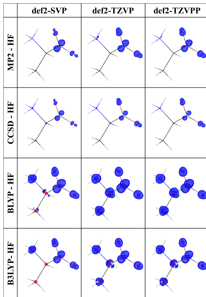
Figure 8. Comparison of the electron densities obtained with the different quantum mechanical methods (references: Hartree-Fock electron distributions) for each adopted basis-set (indicated in the top row). All the electron densities were computed on the IAM structure. Contour level: 0.02 \text{ e bohr}^{-3} ; colors in the difference density plots: blue (positive) and red (negative); the orientation of the molecules corresponds to the one in Figure 2.
