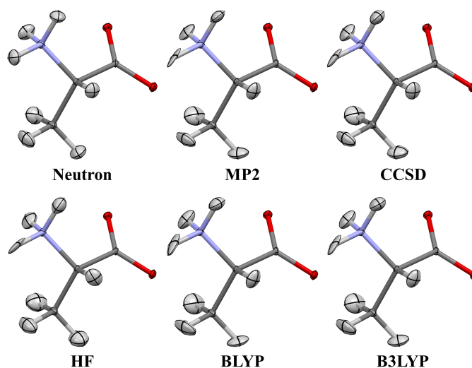
Figure 6. Crystal structures of L -alanine obtained from the refinement of neutron data 80 and from Hirshfeld atom refinements of X-ray data 88 exploiting the basis-set def2-TZVPP. Anisotropic displacement parameters shown with 50% probability. Molecular orientation is identical to the one in Figure 2.
