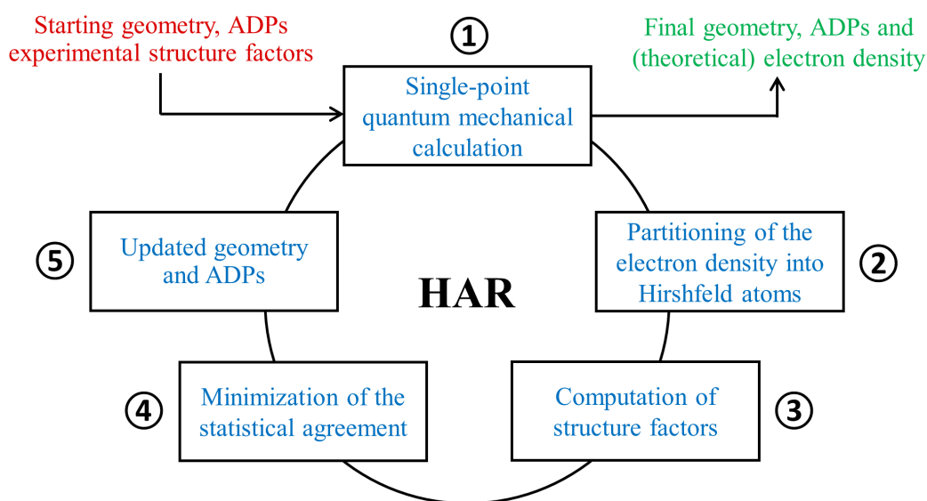
Figure 1. Schematic representation of the Hirshfeld atom refinement algorithm.
