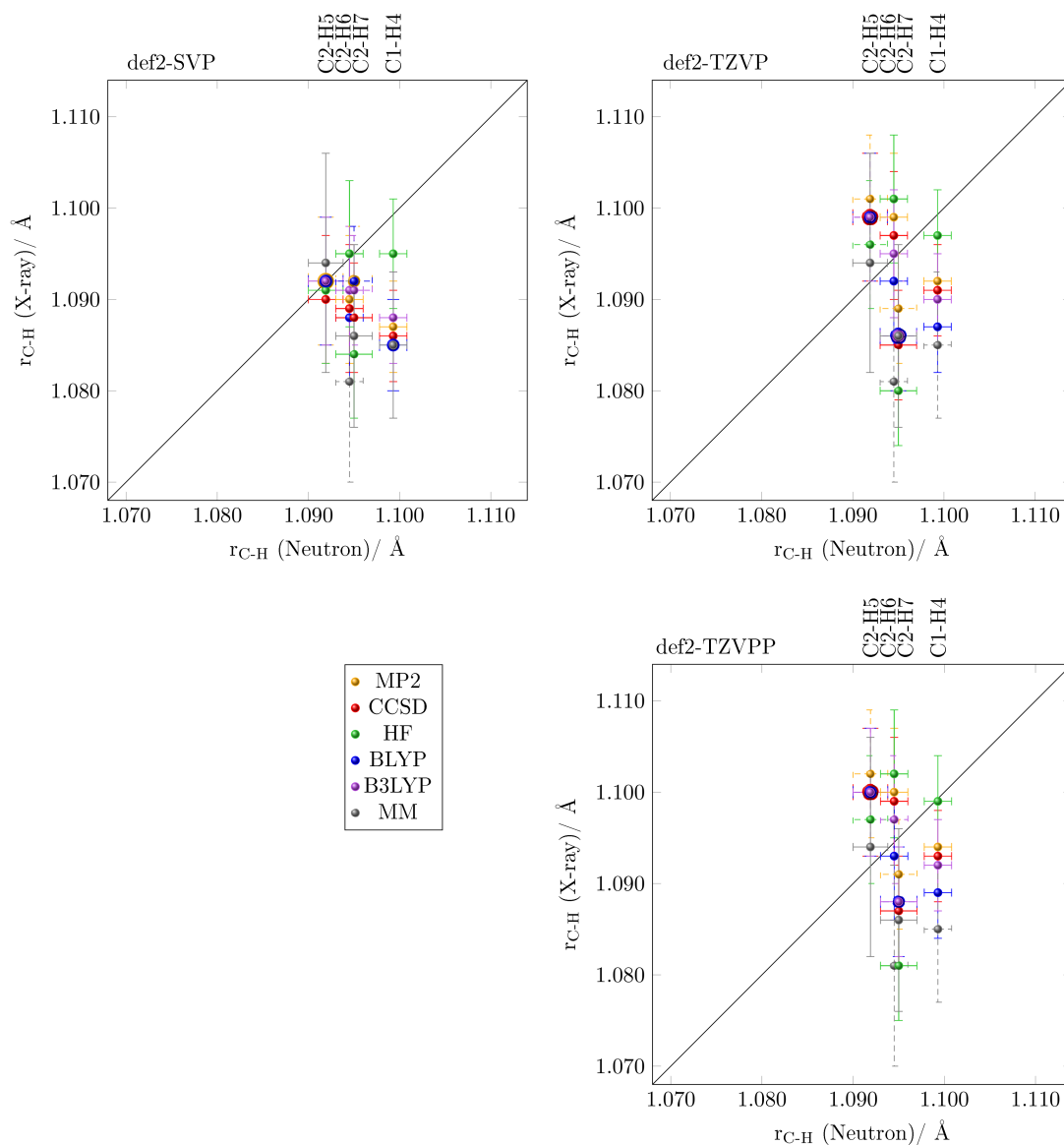
Figure 4. C-H bond lengths in L -alanine for HARs using the def2-SVP (top left), def2-TZVP (top right) and def2-TZVPP (bottom right) basis-sets plotted against neutron C-H bond lengths. C-H bond lengths obtained by Destro and coworkers 89 through a multipole model refinement based on computed hydrogen ADPs are also shown. Vertical bars indicate the experimental errors for the X-ray (HAR or MM) bond lengths, while the horizontal ones represent the uncertainties associated with the neutron results. Bond lengths (in Å) from the IAM refinement: C1-H4: 0.999(9), C2-H5: 0.973(12), C2-H6: 0.997(11), C2-H7: 1.021(11). Bond lengths (in Å) from the MM refinement with isotropic treatment of hydrogen atoms performed by Destro et al. 88 : C1-H4: 1.125(9), C2-H5: 1.086(9), C2-H6: 1.118(9), C2-H7: 1.082(7).
