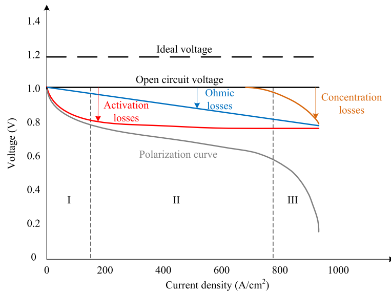
Fig. 2 Various voltage losses and polarization curve of an operating PEMFC [14]
