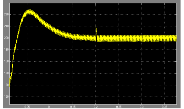
Fig 7. Voltage of DC bus when microgrid works from grid-connected to island
