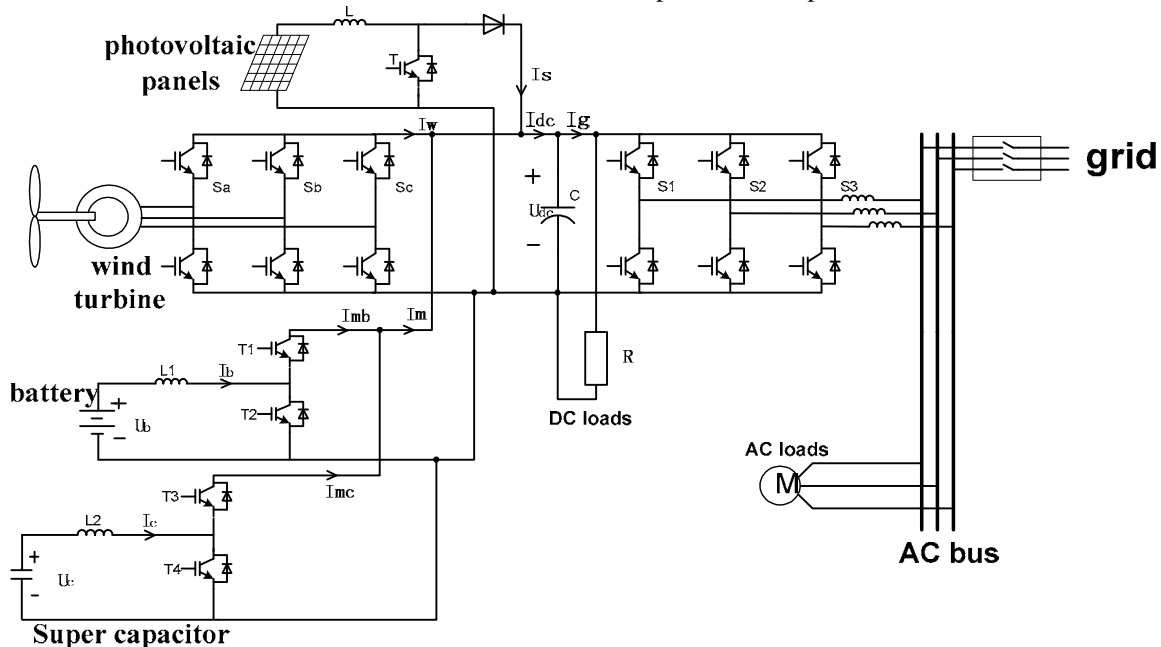
Fig 1. Hybrid DC and AC linked microgrid
