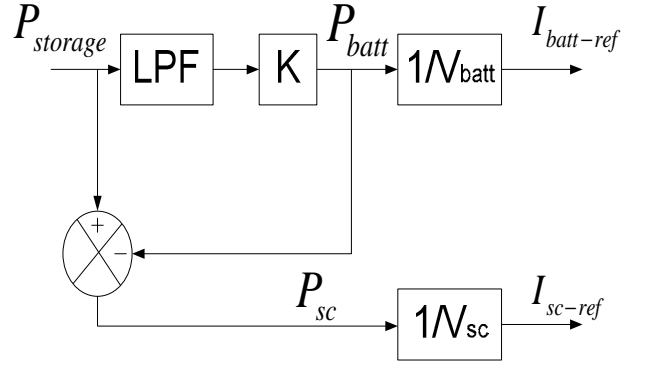
Fig 4. Control strategy of storage system
