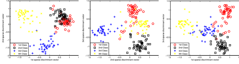
Figure 1: The TOX dataset was projected onto the first three sparse discriminant vectors. The samples in each class are shown by using a distinct symbol.
