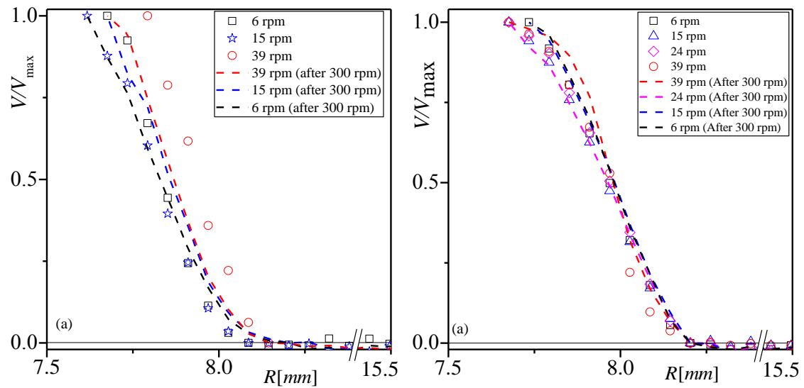
Figure A1. Dimensionless velocity ( V/V_{\max} ) as a function of the radius for (a) 10 wt.%; (b) 15 wt.%.
