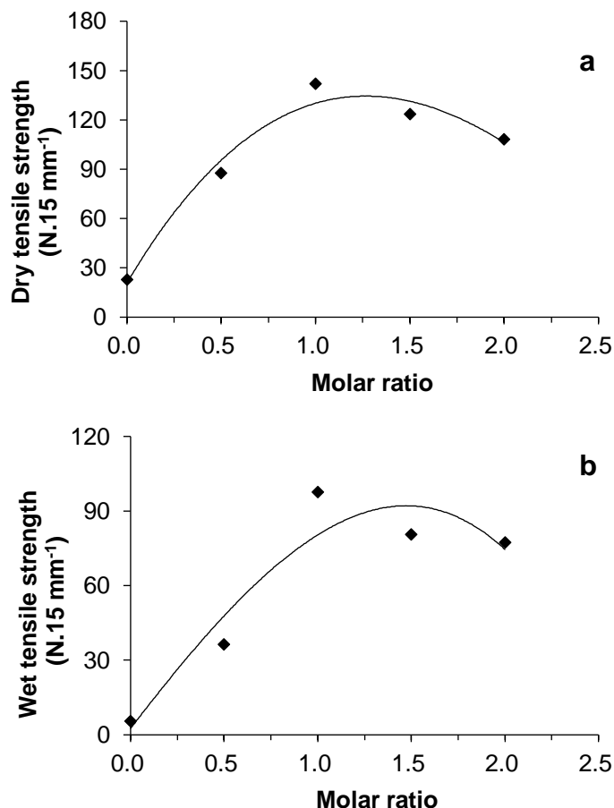
Fig. 2. Effects of the ethylene glycol/melamine molar ratio on the dry tensile strength (a), and wet tensile strength (b) of MF resin-impregnated papers
