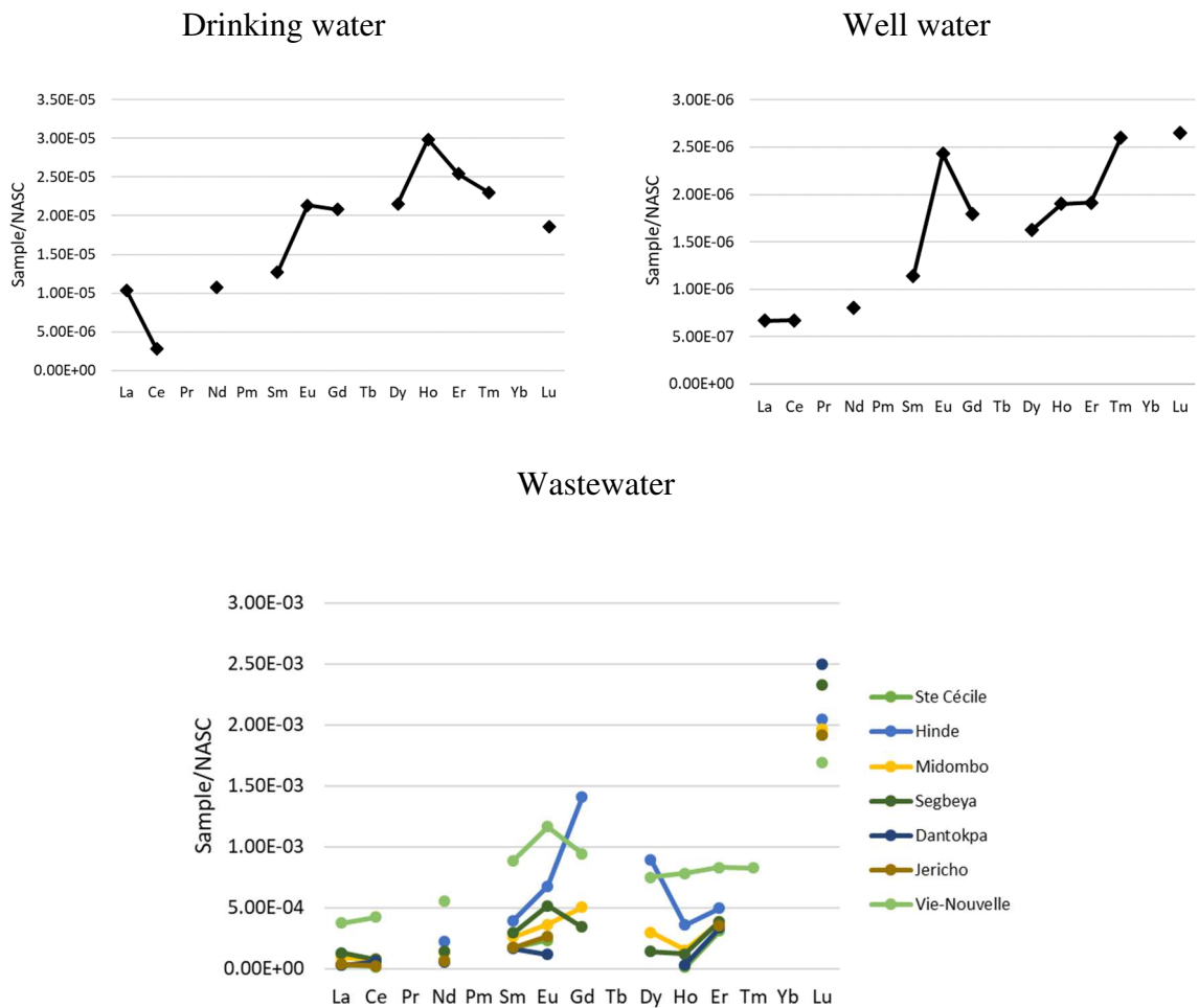
Figure 3: Normalized REE profiles in Cotonou drinking water (average), well water
