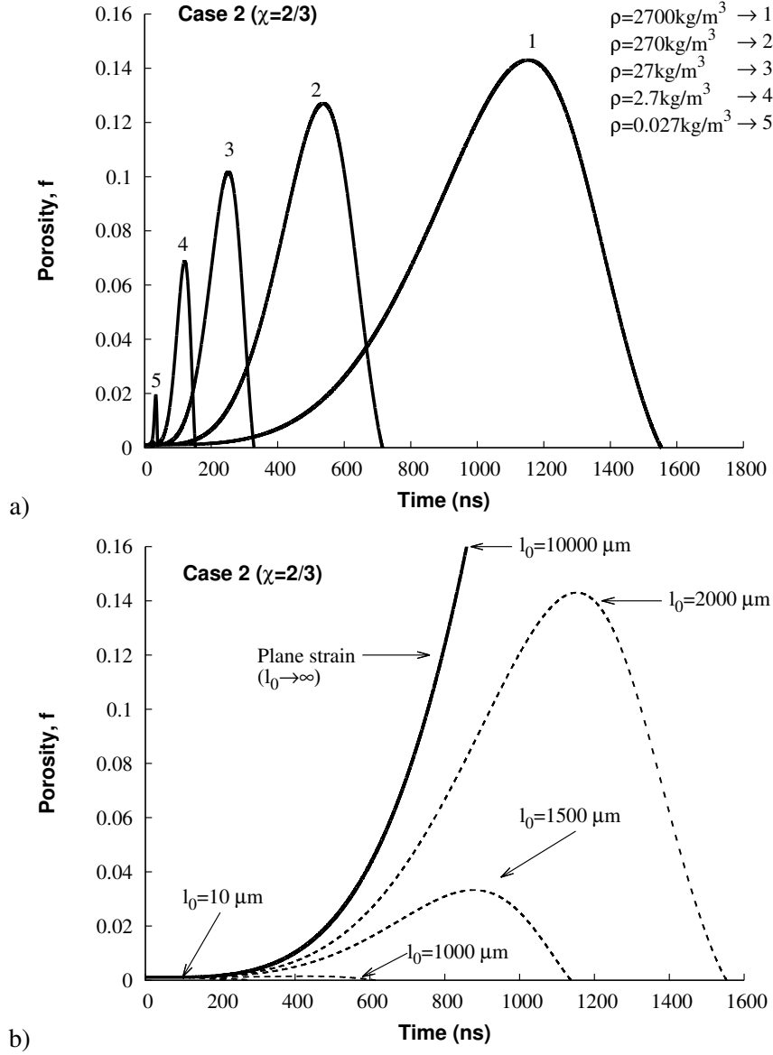
Figure 10: Influence of a) the mass matrix density when l_0=2000\mu\text{m} and b) the initial void length when \rho=2700\text{kg}/\text{m}^3 for Case 2: \Sigma_{11} = \Sigma_{22} = \dot{p}t with \dot{p} = 10\text{MPa}/\text{ns} , \Sigma_{33} = 0 . The other material parameters are displayed in Table 1. The response with l_0 = 10000\mu\text{m} provides the plane strain case of Fig. 2.
