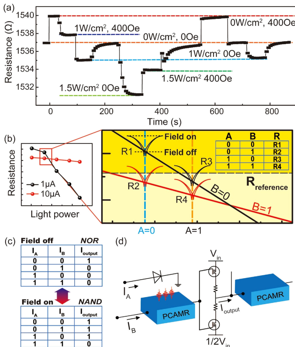
Figure 5. Optically controlled multiresistance states and reconfigurable logics. a) Six different resistance states are realized using different illumination power and magnetic field. b) Two resistance change curves are selected from Figure 2c to illustrate its dependence on measuring current (1 and 10 \mu\text{A} ) when illumination (from 0.5 to 1.6 \text{W cm}^{-3} ) applied. The enlarged picture gives the operation settings of the reconfigurable logics. Light illumination (A) and applied current (B) are defined as two kinds of input signals. The corresponding 0 and 1 settings have been indicated by dashed and solid lines, respectively. Four resistance states achieved through the operation of A and B are summarized in the table. The value under same input signals can still be changed by the magnetic field, marked as the field on and field off states by dotted line. This figure also gives the reference resistance ( R_{\text{Reference}} ) to determine the output 0 and 1. c) The truth table of NOR and NAND operations. With magnetic field applied and removed, the logic can be reversibly switched between them. d) Circuit schematic to realize device concatenability.
