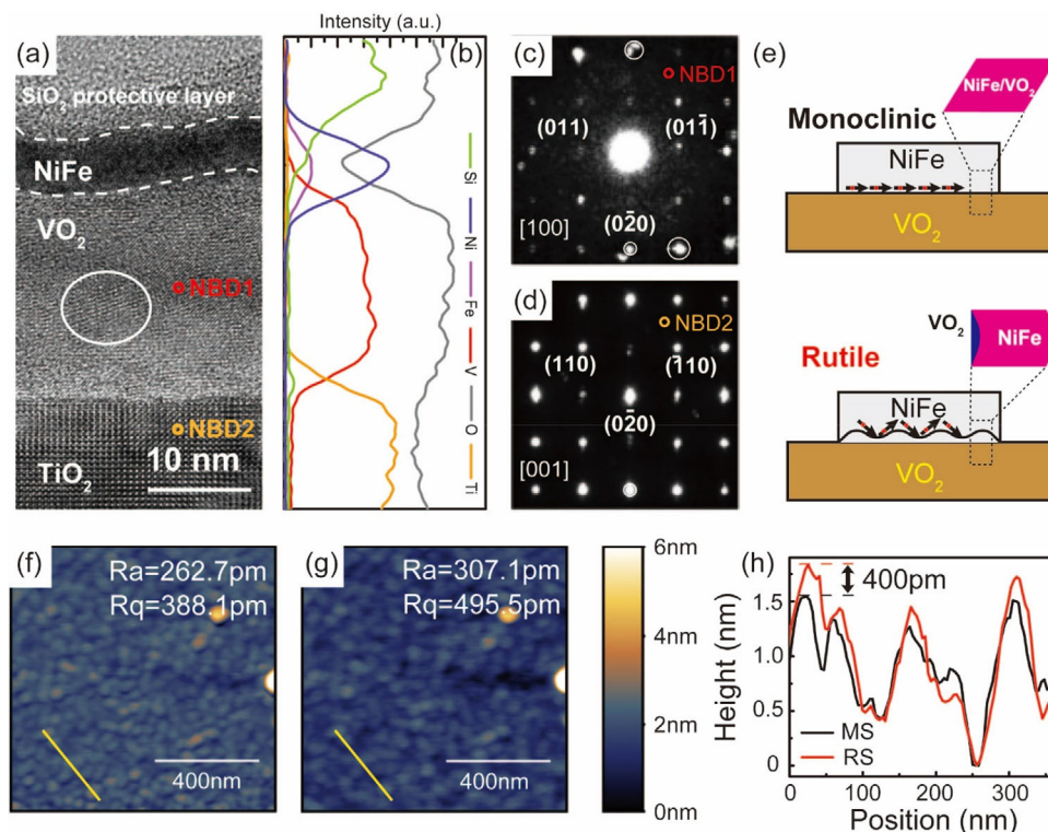
Figure 4. High-resolution transmission electron microscopy (HR-TEM) analysis of the NiFe/VO 2 heterostructure deposited on a TiO 2 (100) substrate. a) Cross-section HR-TEM image of the NiFe/VO 2 heterostructure. Some distortion of the crystal orientation can be detected in the VO 2 layer, as marked in this figure. b) Energy dispersive spectroscopy (EDS) analysis of different elements (Ti, O, V, Fe, Ni, and Si) in the heterostructure. c and d) Nanobeam electron diffraction (NBD) corresponding to NBD1 and NBD2 in (b). e) Schematic diagram of the heterostructure. When the crystal lattice changes, the increased interface roughness causes the spin, which is originally pinned in-plane, to turn to the out-of-plane direction. f and g) Atomic force microscope (AFM) results obtained at 300 and 355 K. The figures also give the average roughness (Ra) and the RMS roughness (Rq) data. A line scanning analysis along the yellow line is given in (h).
