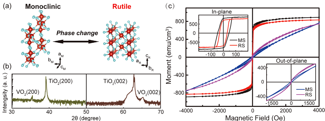
Figure 1. Phase change of VO 2 and characterization of the NiFe/VO 2 heterostructure. a) Schematic illustration of the reversible phase change of VO 2 between monoclinic (M1) and rutile (R) lattice structures. b) XRD \theta - 2\theta scan of the NiFe/VO 2 heterostructure grown on TiO 2 (100) and TiO 2 (001) substrates, suggesting epitaxial growth of the VO 2 layer and polycrystalline growth of the NiFe layer. c) M - H hysteresis loops of the NiFe (5 nm)/VO 2 (20 nm)/TiO 2 (100) sample measured before and after the phase change of VO 2 (MS at 300 K and RS at 360 K). The magnetic field is applied perpendicular (data plotted as circles) and parallel (data plotted as squares) to the surface. The insets give the scanning results over small fields.
