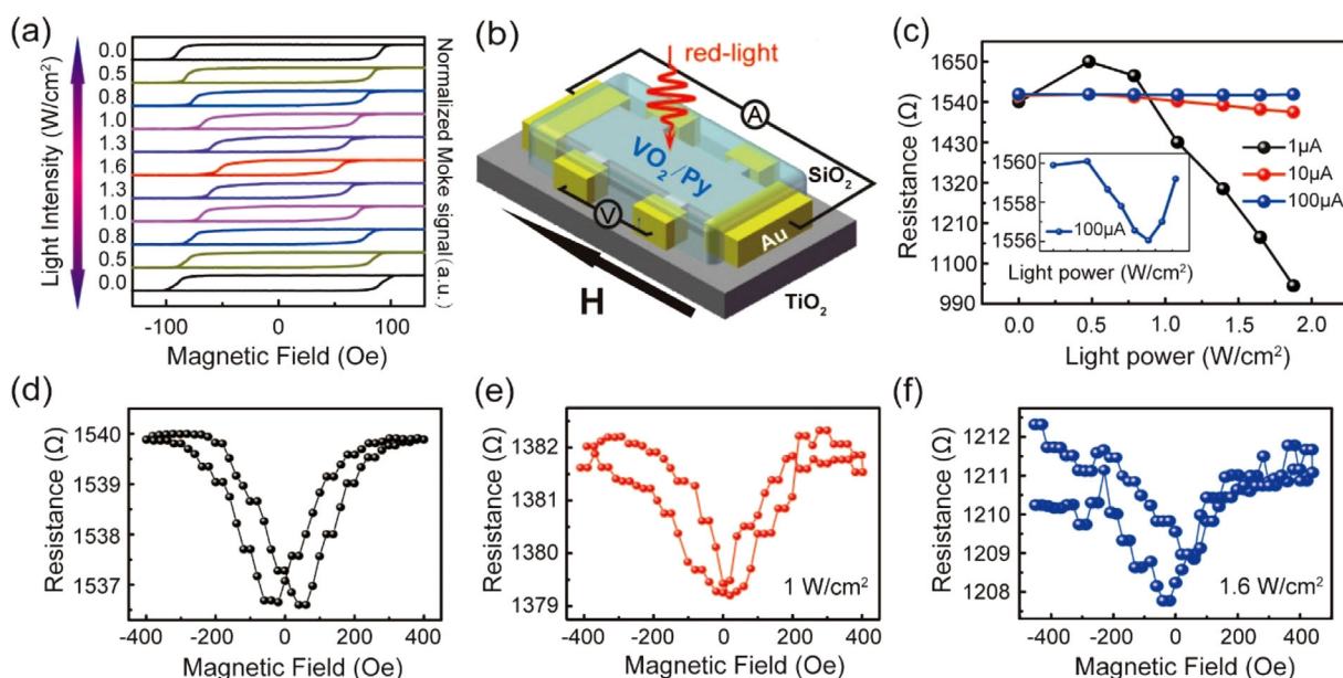
Figure 2. Optically controlled magnetoresistance measurements. a) The hysteresis loops of the sample with different illumination power. b) Schematic drawing of the PCAMR device. Direction of the applied magnetic fields, H , are also presented. c) The device resistance change measured with varied applied current under increasing illumination power. d–f) Comparison of the magnetoresistance of the NiFe (5 nm)/VO 2 (20 nm)/TiO 2 (100) device without (d) and with the illumination of 1 W/cm 2 (e) and 1.6 W/cm 2 (f) red light.
