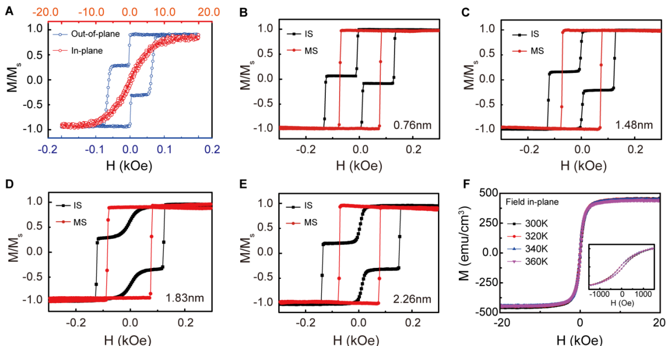
Figure 2. Magnetic properties of [\text{Pt/Co}]_2/\text{VO}_2/[\text{Co/Pt}]_2 heterostructures.
