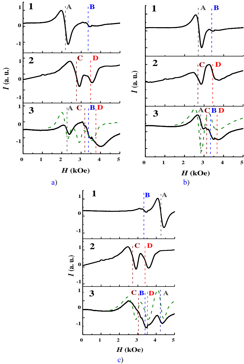
Figure S4. FMR spectrum of CoFeB monolayer without NP's (1), FMR spectrum of Fe/Fe 3 O 4 NP's deposited on Si wafer (2), FMR spectrum of Fe/Fe 3 O 4 NP's deposited on CoFeB monolayer (3), recorded at the angles \theta = 0^\circ (a), 45^\circ (b) and 90^\circ (c) between external magnetic field and perpendicular to the sample's plane. Dashed green line is sum of the independently recorded CoFeB and NP's spectra. Lines A and B correspond to the CoFeB monolayer. Lines C and D correspond to the nanoparticles.
