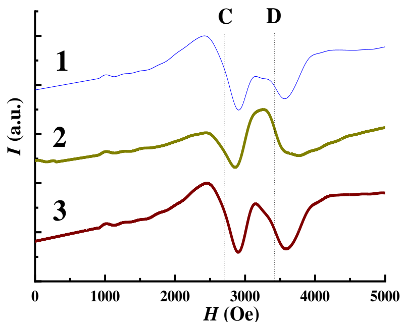
Figure S3. FMR spectra of Fe/Fe 3 O 4 nanoparticles deposited on Si wafer in \theta = 0^\circ (1), 45^\circ (2), 90^\circ (3) orientations of magnetic field in respect to the wafer plane. Vertical lines indicate resonant fields of the lines C and D, correspondently.
