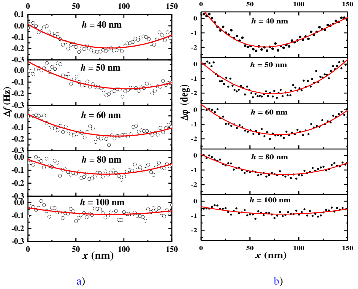
Figure S2. Frequency deviation \Delta f(x) (a), and phase shift \Delta\phi(x) (b), recorded at different heights h 100 nm, 80 nm, 60 nm, 50 nm and 40 nm in MFM mode. Solid lines are approximations by parabola.
