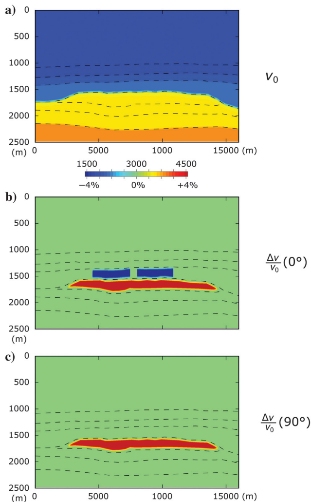
Figure 6. Synthetic dataset. (a) The reference velocity model is heterogeneous and isotropic. The longitudinal wave velocity increases gradually in the shale (the blue area), and it is chosen constant in the carbonate (the orange area). The dimensions are in meters. The ashed lines correspond to reflectors. (b) Vertical velocity change. (c) Horizontal velocity change.
