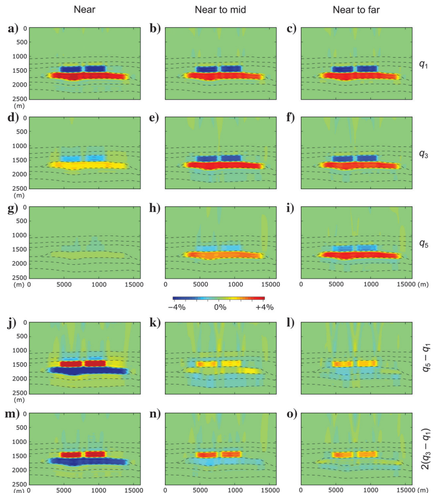
Figure 7. Anisotropic velocity changes retrieved by anisotropic reflection traveltome tomography. The columns represent the different offset acquisitions. Rows represent the anisotropic velocity change parameters q_1 , q_3 , and q_5 and the algebraic formula q_5 - q_1 ( \epsilon ) and 2(q_3 - q_1) ( \delta ). The parameters q_2 and q_4 are inverted but are not presented because they are equal to zero. The terms q_1 and q_5 must be compared with Figure 6b and 6c.
