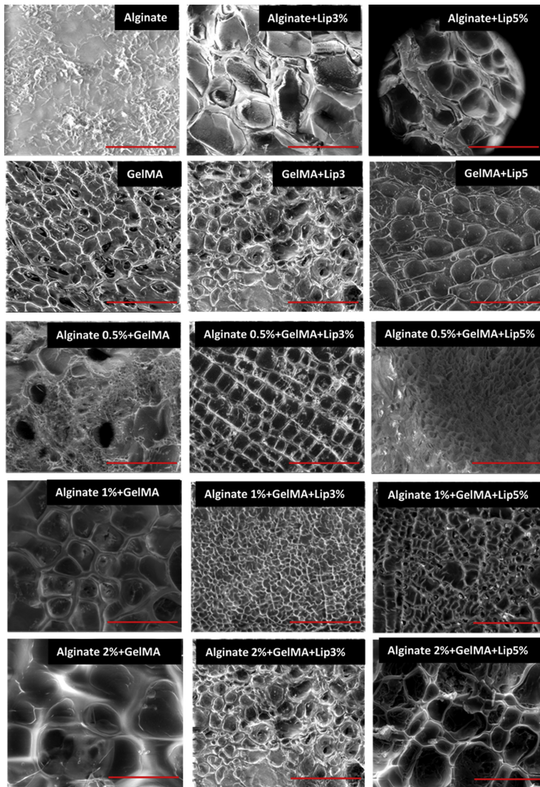
Fig. 1. SEM images of 3D hydrogels of various systems before and after functionalization. (Scale bar = 300 \mu m). 3D = three-dimensional; SEM = scanning electron microscopy; GelMA = gelatin methacryloyl. S = \mu
