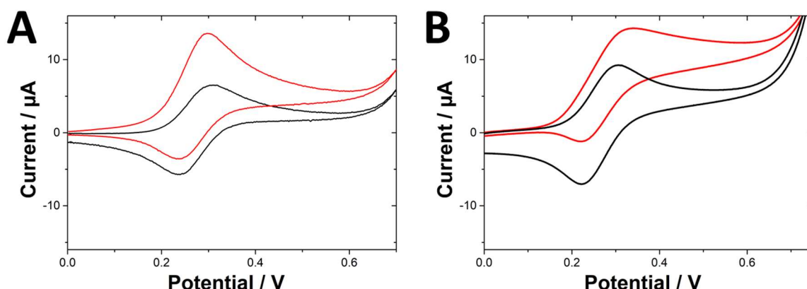
Figure 1: Cyclic voltammetry at a mesoporous silica film electrode of 0.5 mM of \text{Fc}(\text{MeOH})_2 in the absence (black curve) and in the presence (red curve) of (A) 1.25 mM cysteine and (B) 1.49 mM glutathione. \nu = 10 \text{ mV s}^{-1} .
