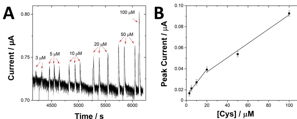
Figure 6: (A) Chronoamperograms obtained for increasing concentrations of cysteine (3-100 \mu\text{M} ). E_{applied} = + 0.65 \text{ V} ; flow rate was 1 \text{ mL min}^{-1} . (B) Calibration curve showing peak current as a function of cysteine concentration.
