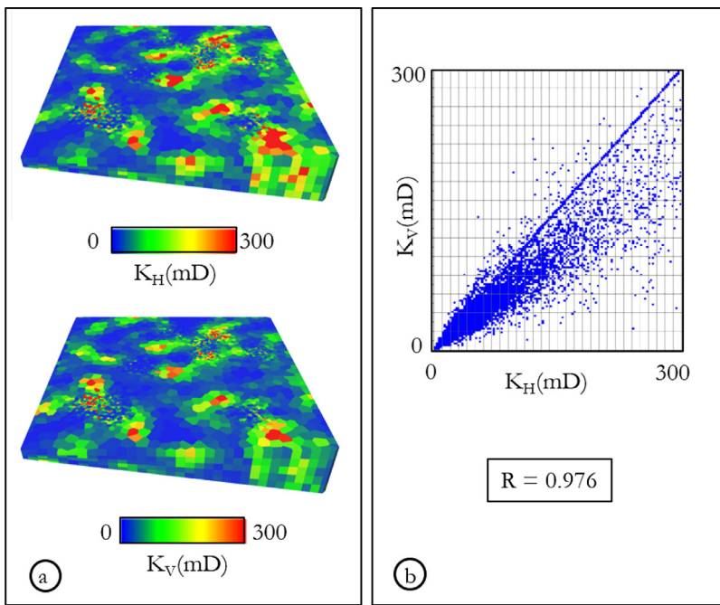
Fig. 13. a) Vertical and horizontal permeability fields on the toy example. b) Cross-plot K_H vs. K_V , K_V being globally inferior to K_H .
