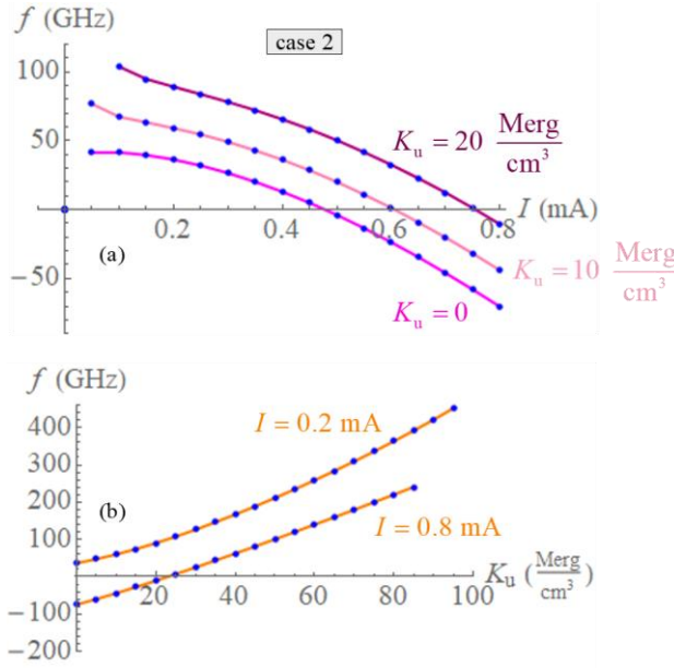
Figure S14: (a) Frequency-current characteristics for several illustrative values of perpendicular-magnetocrystalline-anisotropy energy density K_u of the free layer in case 2. (b) Precessional frequency as a function of K_u for two different applied current amplitudes.
