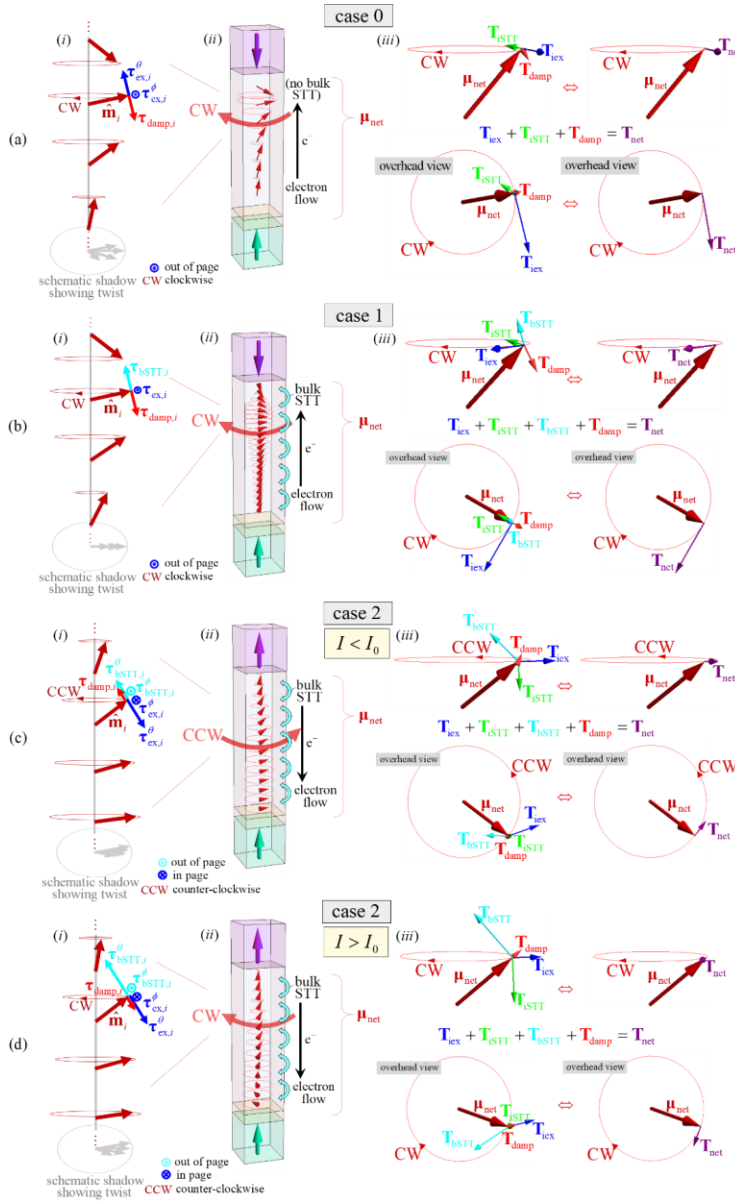
Figure 4: Illustrations of the competitions between local torques \mathbf{T}_i 's acting on an arbitrary interior spin \mathbf{m}_i , and of net torques \mathbf{T} 's acting on the net free-layer magnetic moment \mathbf{\mu}_{net} , during steady state CW precession for cases 0, 1, and 2.
