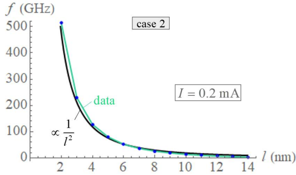
Figure S13: Frequency of precession as a function of free-layer length for a given applied electric current in case 2, showing an inverse square dependence.
