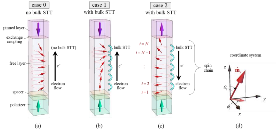
Figure 1: Schematic illustration of an all-perpendicular spin valve in the three cases considered: (a) case 0, (b) case 1, (c) case 2. In cases 0 and 1, the polarizer and pinned layer magnetizations are oppositely oriented and electron flow is in the direction from polarizer to pinned layer. In case 2, the magnetizations of pinned layer and polarizer are equally oriented, and the electron flow is in the reverse direction. In case 0, the electron flow within the bulk of the free layer is not spin polarized, while in cases 1 and 2 it is. The free layer magnetization is modeled as a chain of spins, with the adopted spin-numbering scheme shown in Fig. 1c. Figure 1d shows the coordinate system with respect to which the direction of each spin \vec{i} is represented in terms of the polar and azimuthal angles, \theta_i and \phi_i , respectively.
