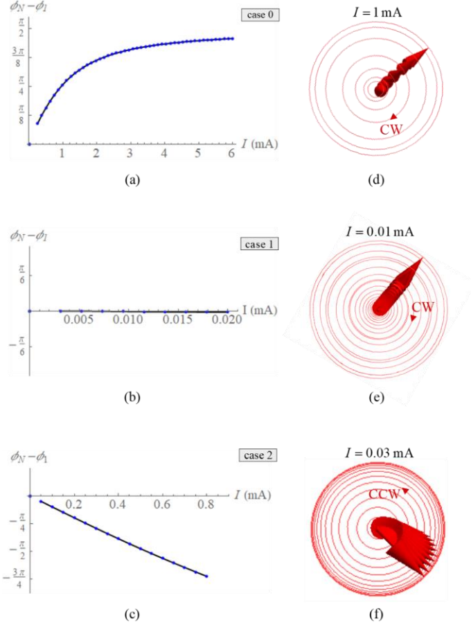
Figure 6: (a-c) The azimuthal angle difference, \phi_N - \phi_I , between the topmost and the bottommost free-layer spin as a function of applied current for cases 0, 1, and 2. The angle difference reflects the twist in the spin chain, which monotonically changes with applied current in cases 0 and 2, while it is absent in case 1. (d-f) An overhead view of the free layer spins at a given current showing the developed twist in the spin change. (A careful comparison of the positions of the arrow tips with respect to their circular traces reveals that in case 0 \phi_N - \phi_I \approx 45^\circ for the specified current value.)
