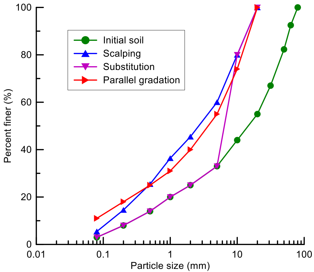
Figure 1: Modification of the grain size distribution curve for the three different approaches (initial soil: d_{max} = 80 mm and reconstituted soils: d_{max} = 20 mm)
