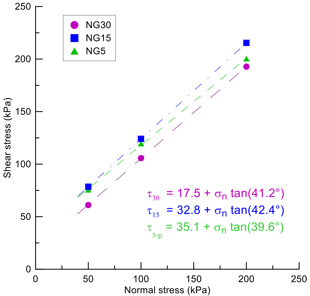
Figure 11: Failure envelopes of NG specimens tested at \rho_d = 2 \text{ Mg/m}^3 .
