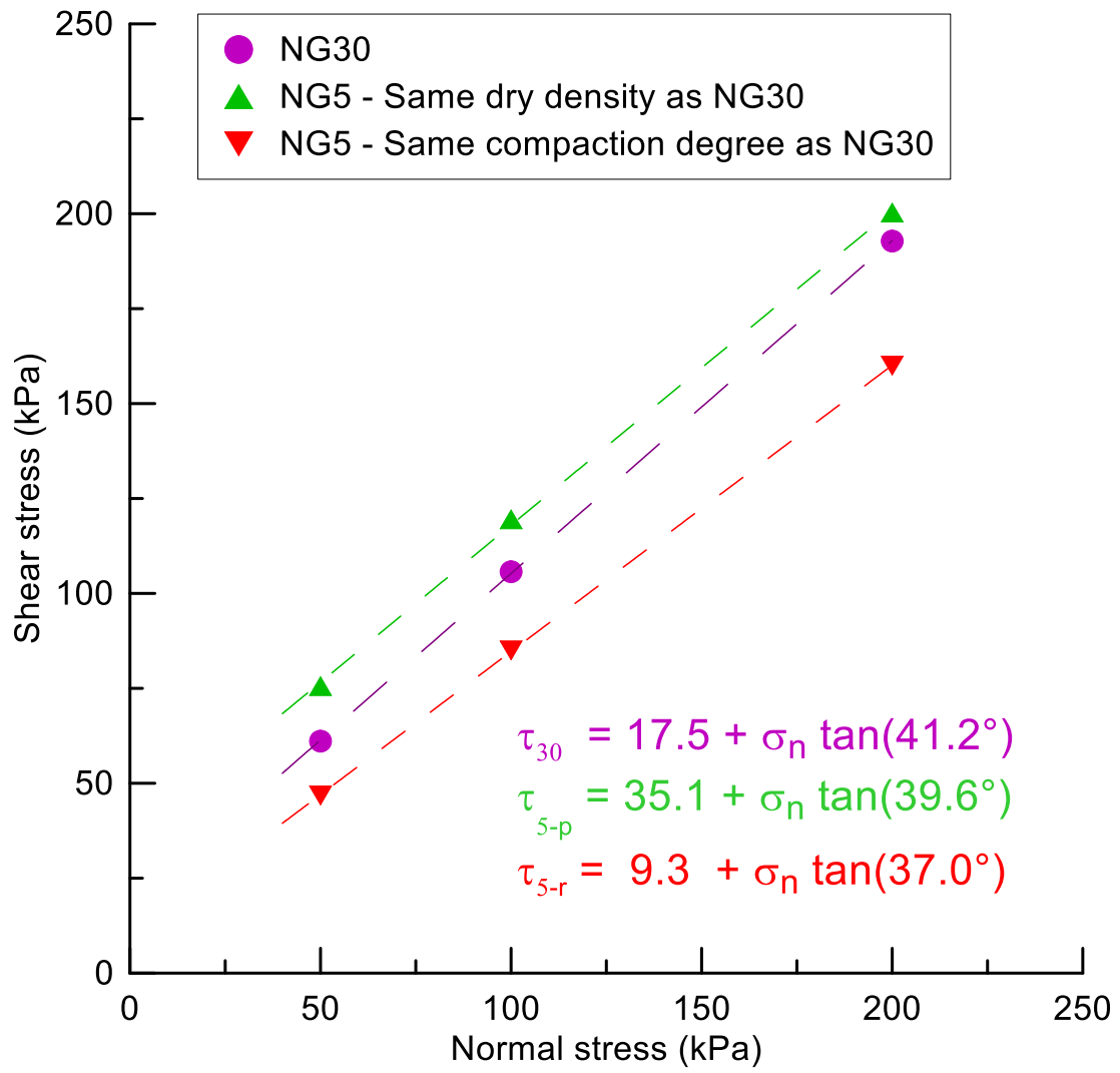
Figure 9: Failure envelopes of NG30 and NG5 (NG30: \rho_d = 2 \text{ Mg/m}^3 and NG5: \rho_d = 2 or 1.83 \text{ Mg/m}^3 ).
