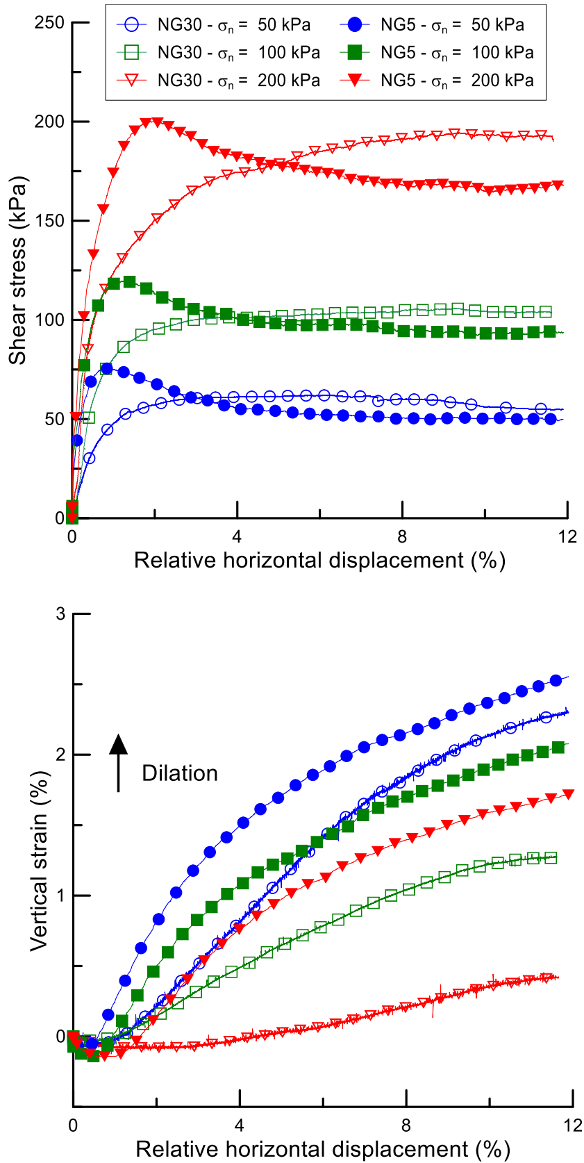
Figure 8: Shear stress-relative horizontal displacement and volume variation curves of NG5 and NG30 at \rho_d = 2 \text{ Mg/m}^3 .
