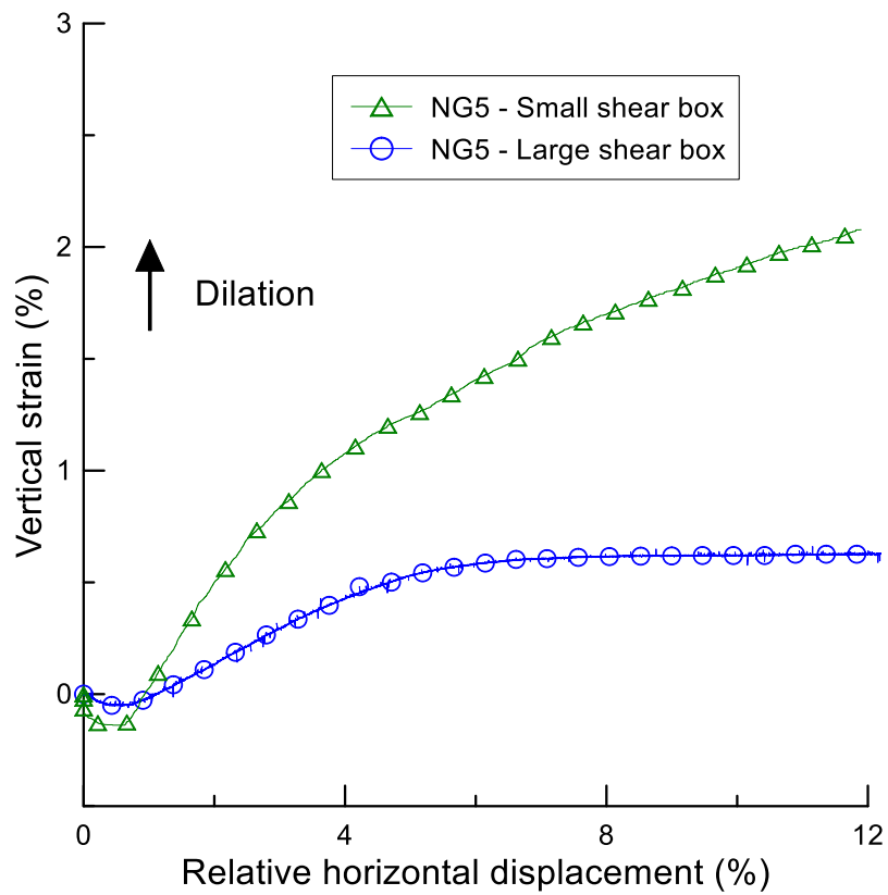
Figure 4: Effect of specimen dimensions on the shear strength of NG5 ( \sigma_n = 100 kPa).
