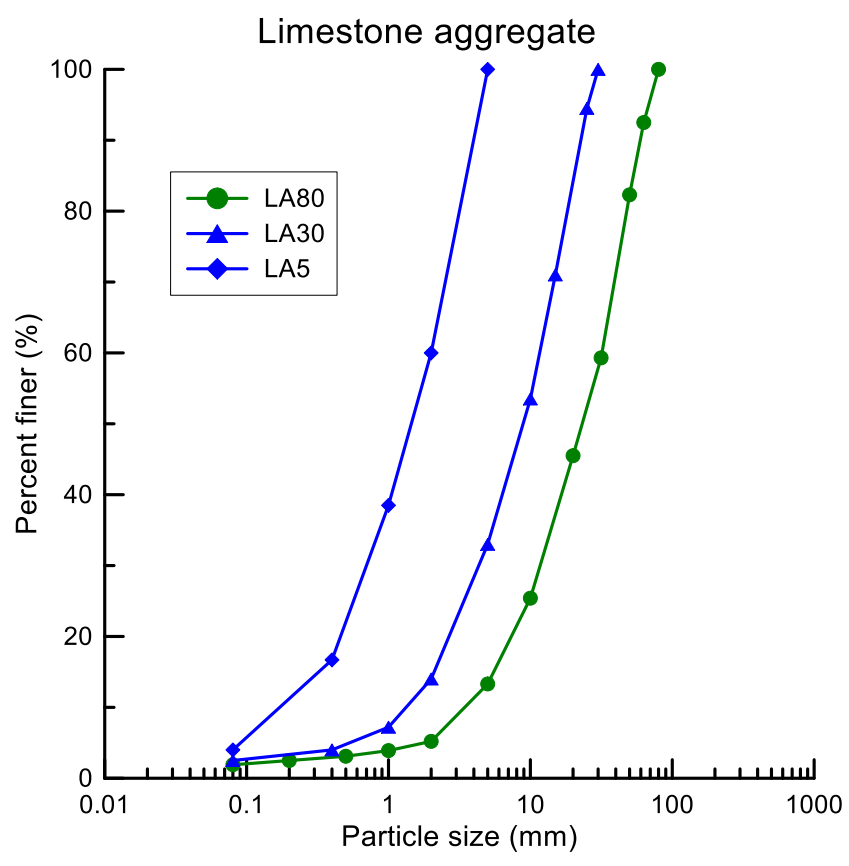
Figure 2: Grain size distribution curves of the studied soils.
