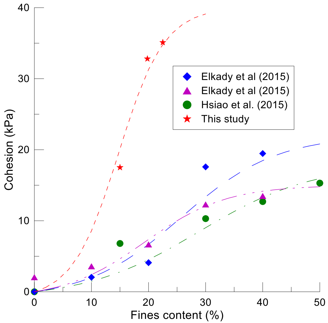
Figure 12: Variation of the cohesion with the fines content.
