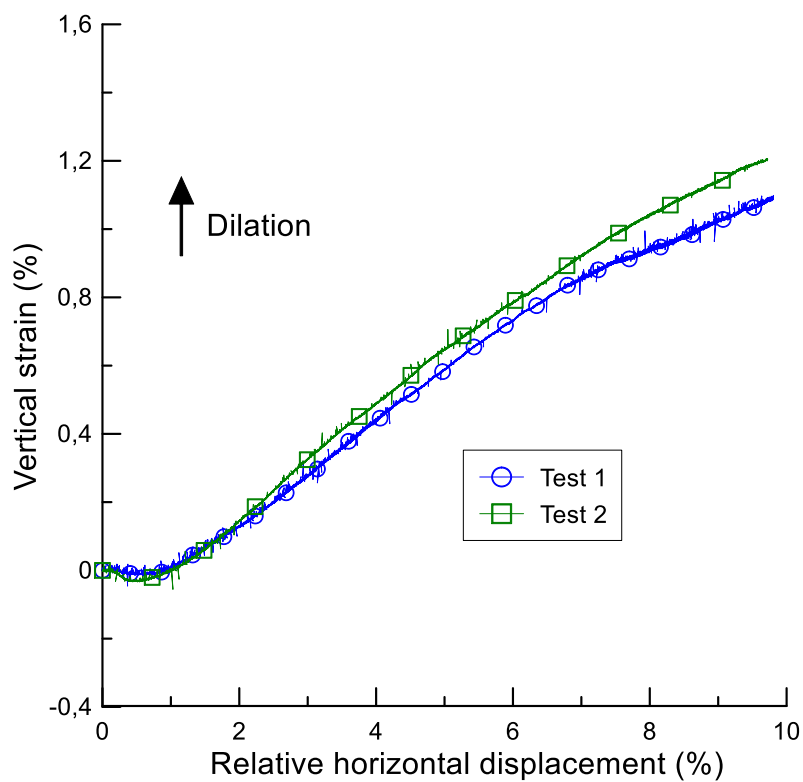
Figure 3: Repeatability tests on NG30 under 100 kPa of normal stress in the large shear box.
