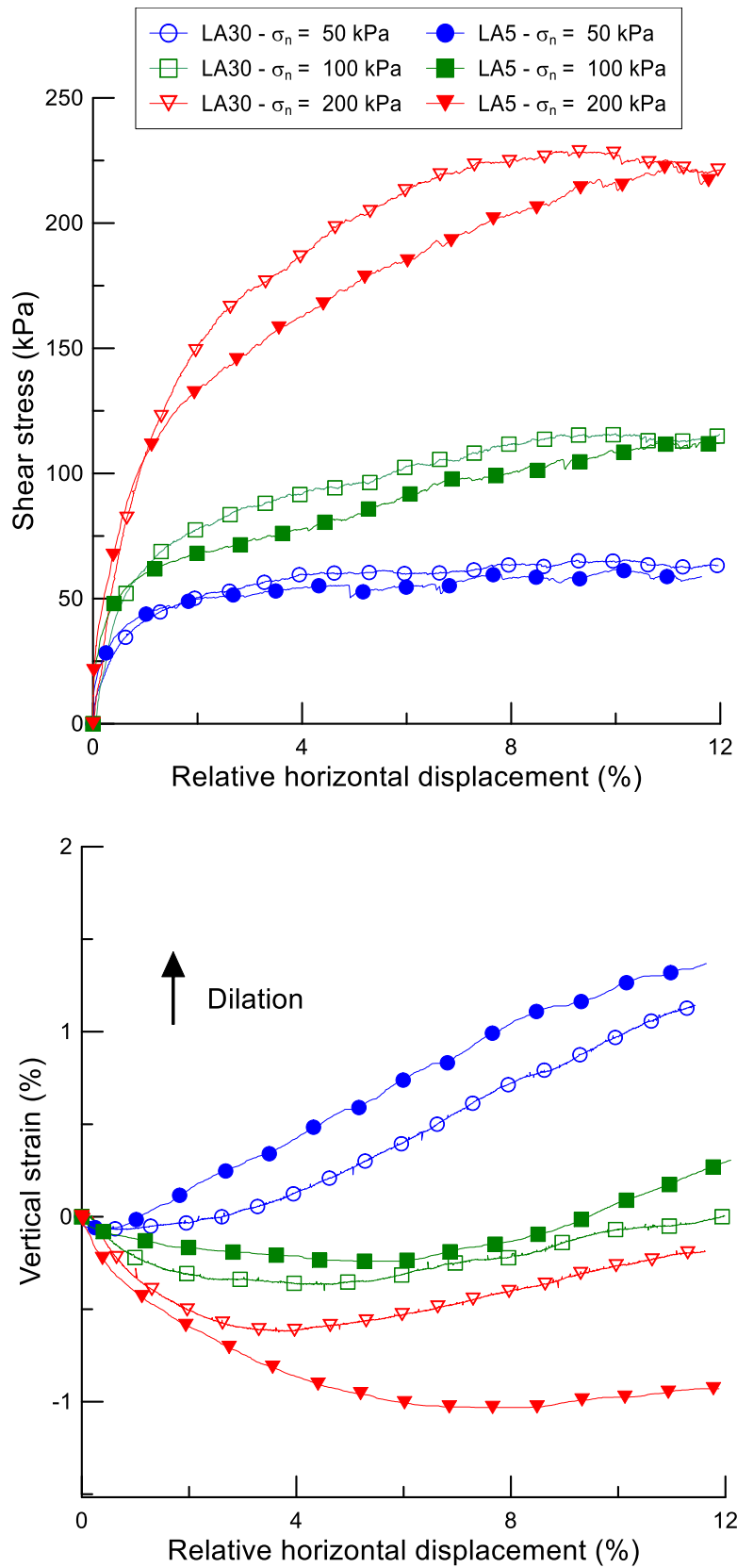
Figure 5: Shear stress-relative horizontal displacement and volume variation curves of LA5 and LA30 at \rho_d = 1.73 \text{ Mg/m}^3 .
