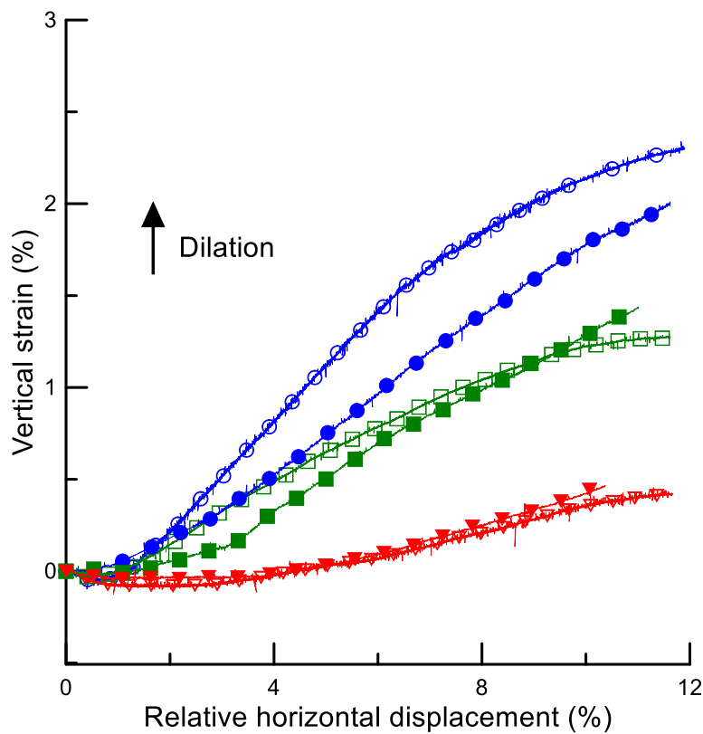
Figure 10: Shear stress-relative horizontal displacement and volume variation curves of NG15 and NG30 at \rho_d = 2 \text{ Mg/m}^3 .
