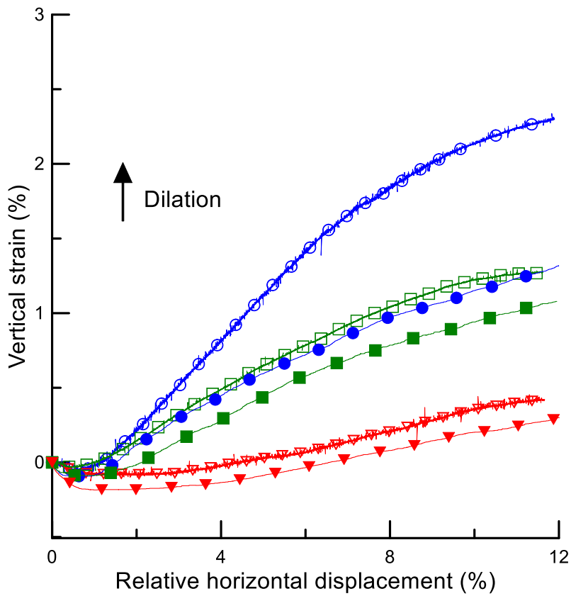
Figure 7: Shear stress-relative horizontal displacement and volume variation curves of NG5 and NG30 at 94% of compaction degree (NG30: \rho_d = 2 \text{ Mg/m}^3 and NG5: \rho_d = 1.83 \text{ Mg/m}^3 ).
