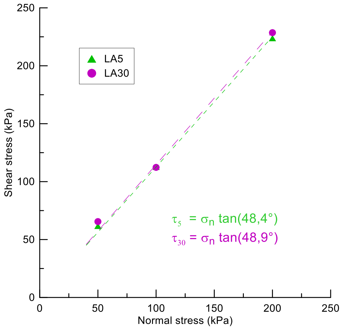
Figure 6: Failure envelopes of LA5 and LA30 at \rho_d = 1.73 \text{ Mg/m}^3 .
