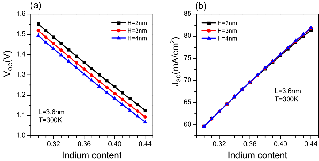
Figure 6: Open-circuit voltage variation as a function of In -content x (a) and photo-generated current density variation versus In -concentration (b). The dot size and the temperature are fixed at L = 3.6 nm and T = 300 K , respectively and the inter-dot spacing takes three values: H = 2, 3 and 4 nm .
