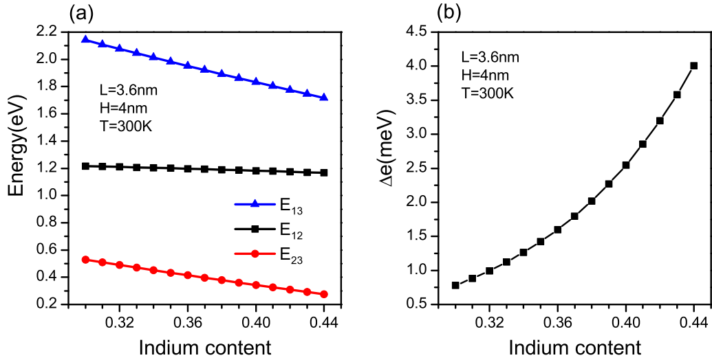
Figure 5: Variation of the band gap E_{13} , sub-bands E_{12} and E_{23} (a), IB width (b) at fixed L = 3.6 nm , H = 4 nm and T = 300 K , versus In -concentration x .
