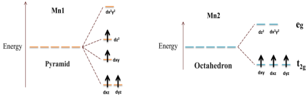
Figure 4: Energy levels and filling of 3d manganese orbitals in a pyramidal (left) and octahedral (right) environment.
