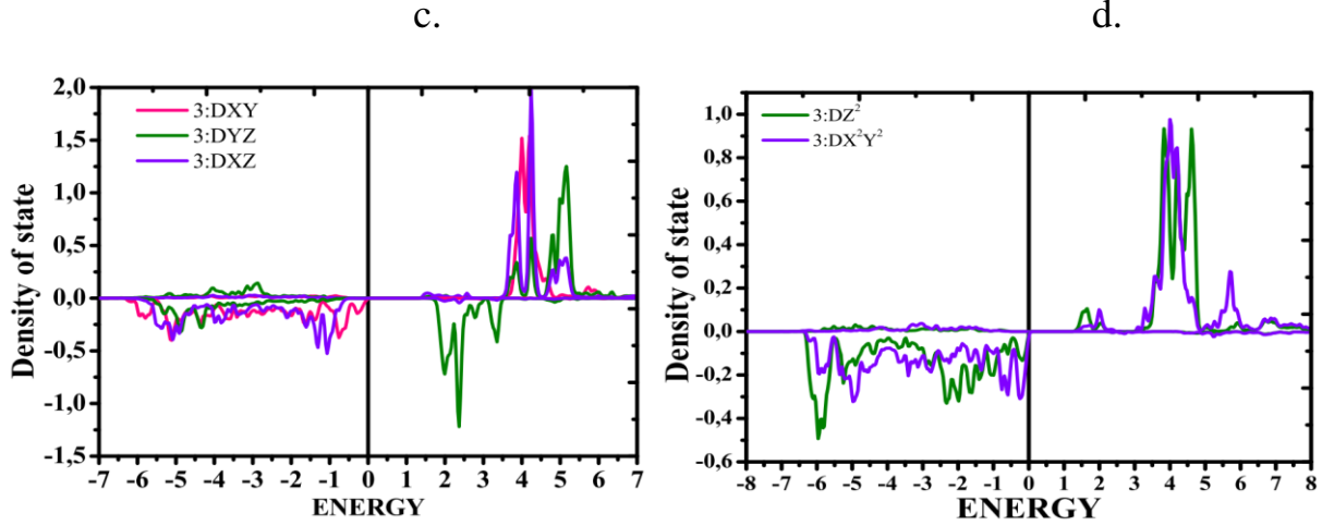
Figure 5: The density of state as a function of energy (eV), of Mn1 (number 2) and Mn2 (number 3) atoms, (a) dxy, dxz and dyz states, (b) dz 2 and dx 2 y 2 states for Mn1 atoms, and (c) dxy, dxz and dyz states, (d) dz 2 and dx 2 y 2 states for Mn2 atoms.
