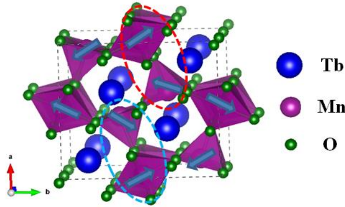
Figure 1: Orthorhombic structure of \text{TbMn}_2\text{O}_5 , the blue arrows indicate the magnetic structure of manganese ions.
