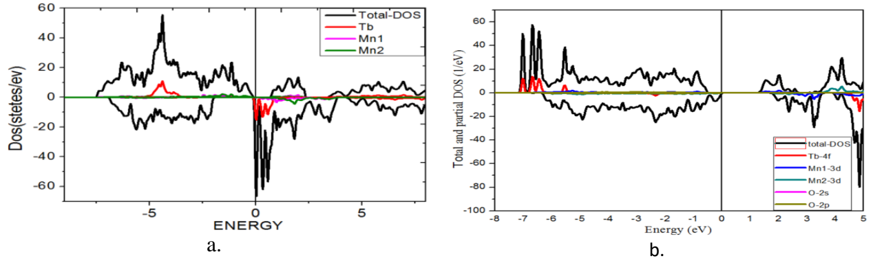
Figure 3: (a) Total density of states for TbMn 2 O 5 with the GGA approximation. (b) Total and partial density of states for TbMn 2 O 5 with the GGA+U approximation.
