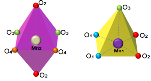
Figure 2: Basic structural units of distorted Mn1O 5 octahedra and Mn2O 6 square pyramid
