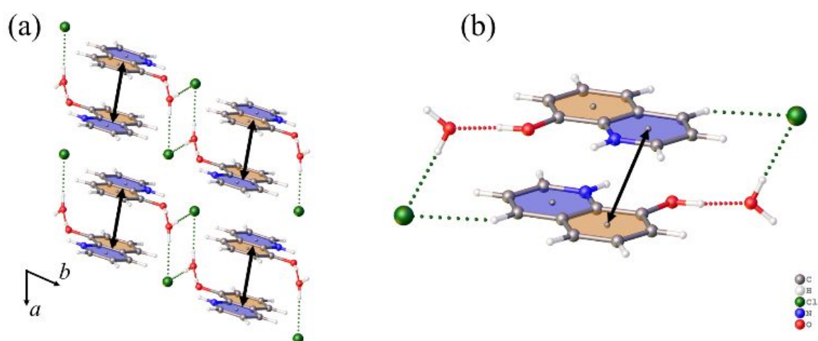
Figure 3. (a) Crystal packing of the HQ.Cl salt projected along the [001] direction, and (b) structural arrangement within organic cation dimers. Black arrows depict the intra-dimer \pi - \pi stacking interactions, while N-H...Cl, C-H...Cl and O-H...OH 2 hydrogen bonds are shown as dotted lines.
