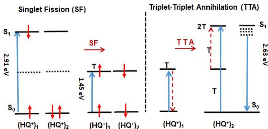
Figure 8: Schematic representations of the sensitizer free TTA- UC mechanism: The fission of two singlet states into two triplet states occurring into two interacting \text{HQ}^+ cation is followed by an emission via triplet – triplet annihilation (TTA) .
