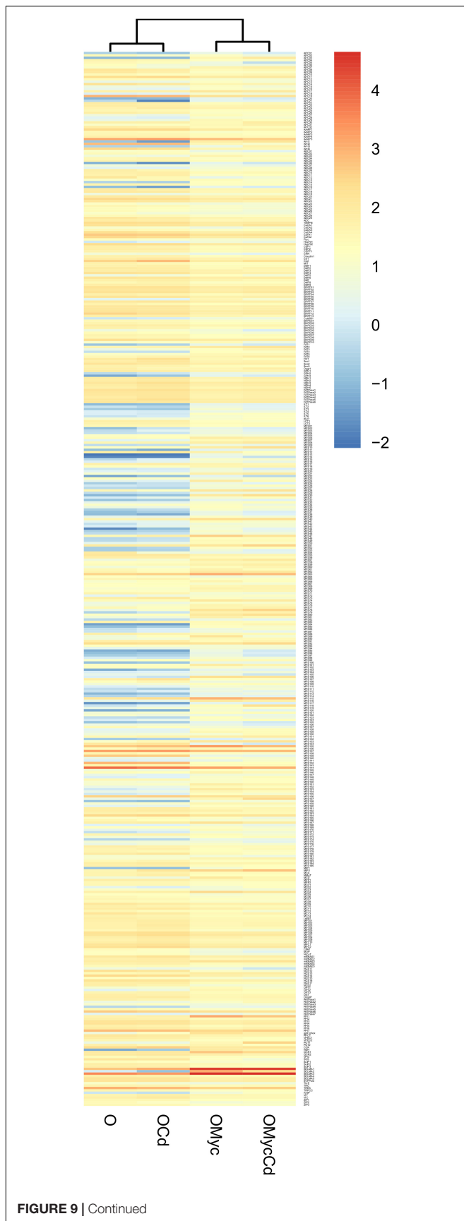
FIGURE 9 | Cd-exposure and mycorrhizal effects on the expression pattern of O. maius Zn putative TPs families. The figure represents a heatmap visualization and single hierarchical clustering of the regulated ( p < 0.05 ) putative TPs of O. maius Zn. Rows are ordered by TPs family composition whereas columns are ordered by hierarchical clustering. The intensity of the color is representative of the \text{Log}_{10} of mean expression value of each gene. On the right, the color-key expression code.
