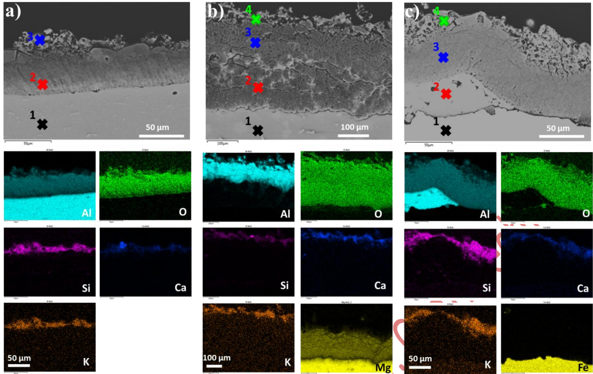
Figure 5: Cross-sections SEM micrographs and the corresponding EDX element maps for the duplex coatings grown on a) bulk Al 1050 (Al+CS0μm+PEO35min), b) Mg EV31 (Mg+CS66μm+PEO20min) and c) S235 steel substrate (St+CS80μm+PEO20min). Coloured crosses indicate the localization of EDX measurements and element quantification given in Fig. 6 and Tables 6, 7 and 8.
