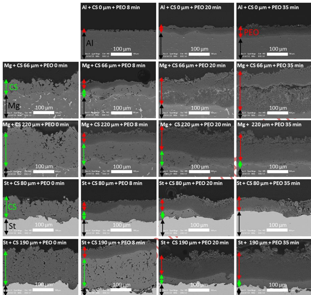
Figure 3: Cross-section SEM micrographs of the cold-sprayed and PEO processed samples for different PEO processing time. Reference name of each sample is given in Table 4. Black arrows indicate the substrate (Al, Mg or Steel), green arrows indicate the cold-sprayed Al coating and red arrows indicate the PEO coating.
