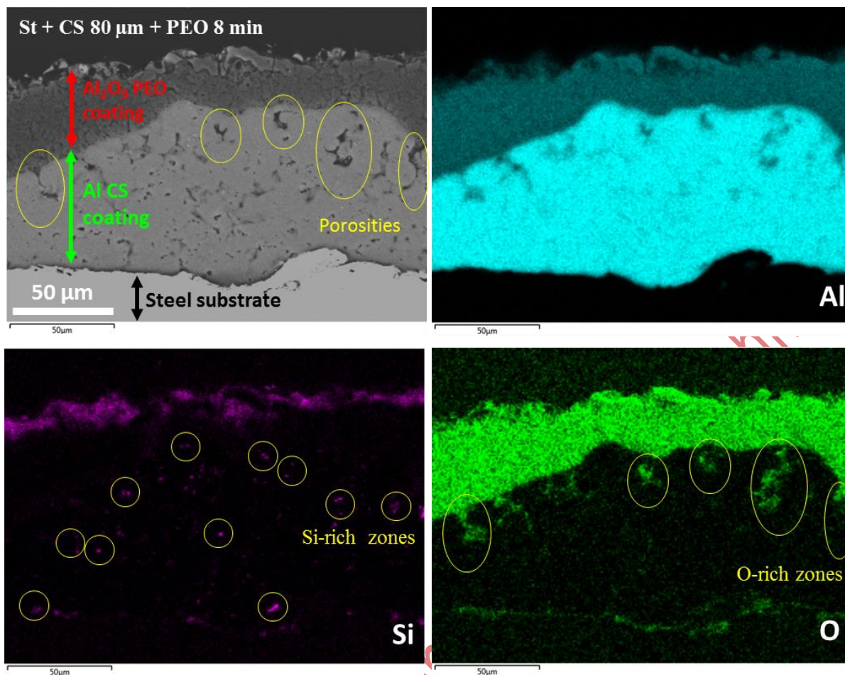
Figure 8: Cross-sections SEM micrographs and corresponding EDX element maps (Al, Si and O) of a PEO coating grown on a pre-deposited steel substrate (St+CS80 \mu\text{m} +PEO8min).
