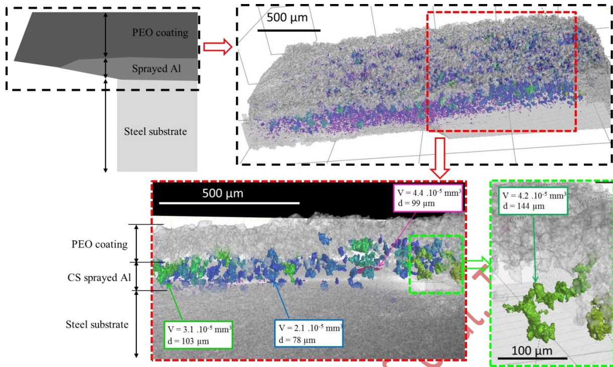
Figure 9: X-ray micro-tomography images of a PEO coating grown on a steel substrate (St+CS190 \mu\text{m} +PEO35min). V is the volume of porosities. d is the path length of the porosities.
